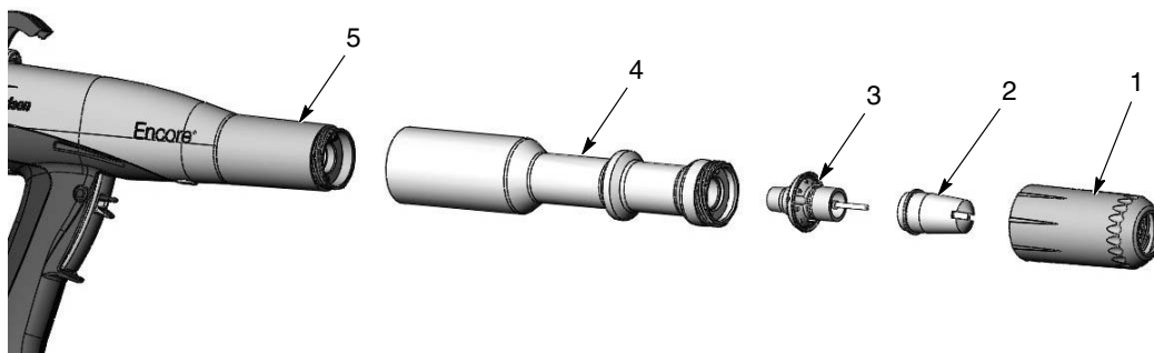
Figure 2 Installation de la lance prolongatrice
