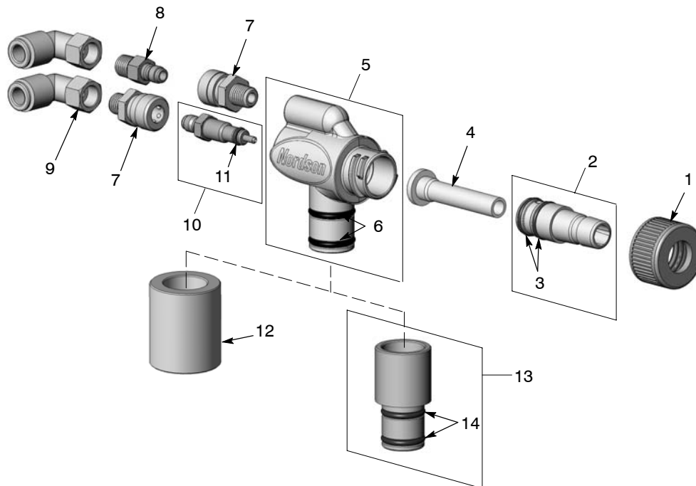
Abb. 6-9 Pumpe
