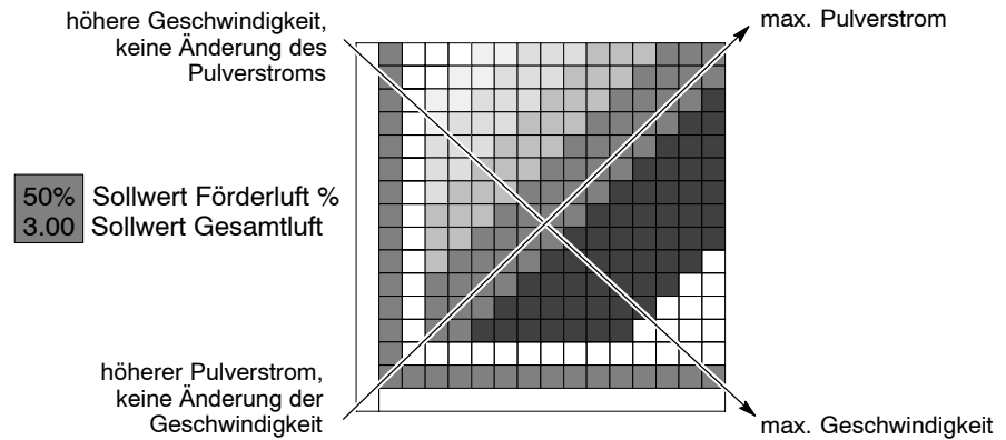
Abb. 3-17 Smart Flow Tabellen lesen
