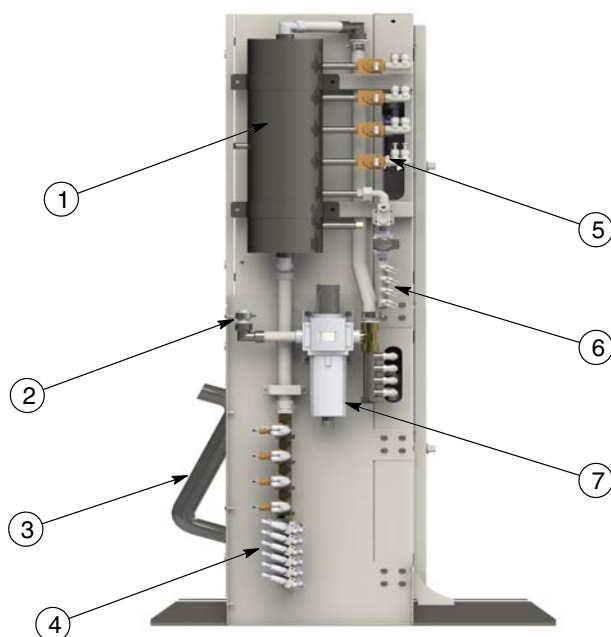
Fig. 2 Pneumatics major component overview
