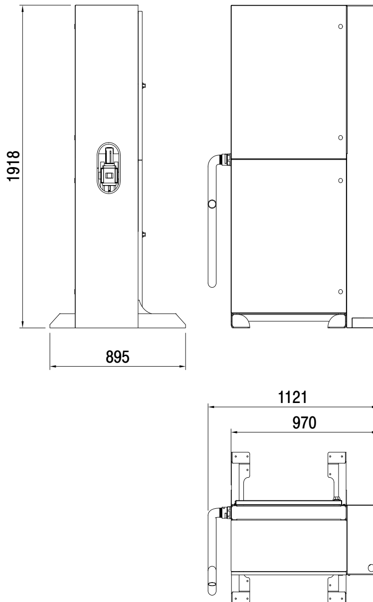
Fig. 3 Overall dimensions
