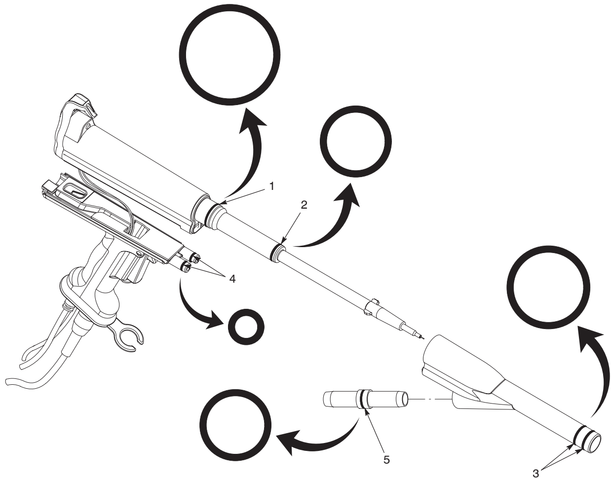
Figure 1 Sure Coat Manual Powder Spray Gun Seals Kit
