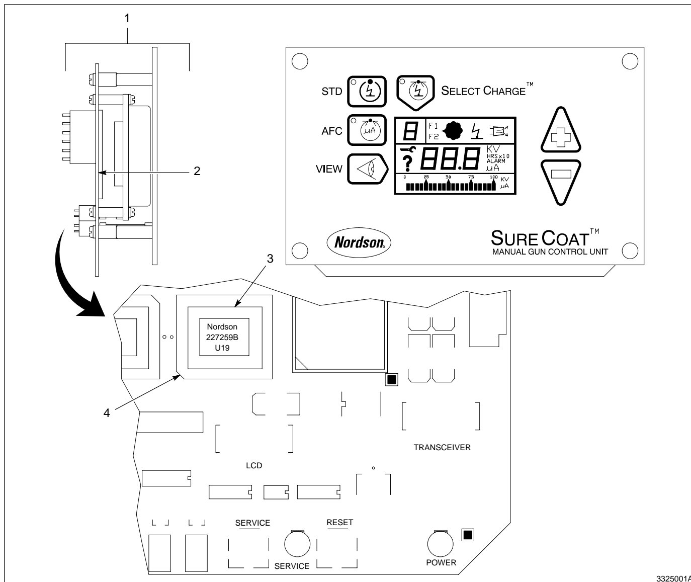
Fig. 1 Controller board location
