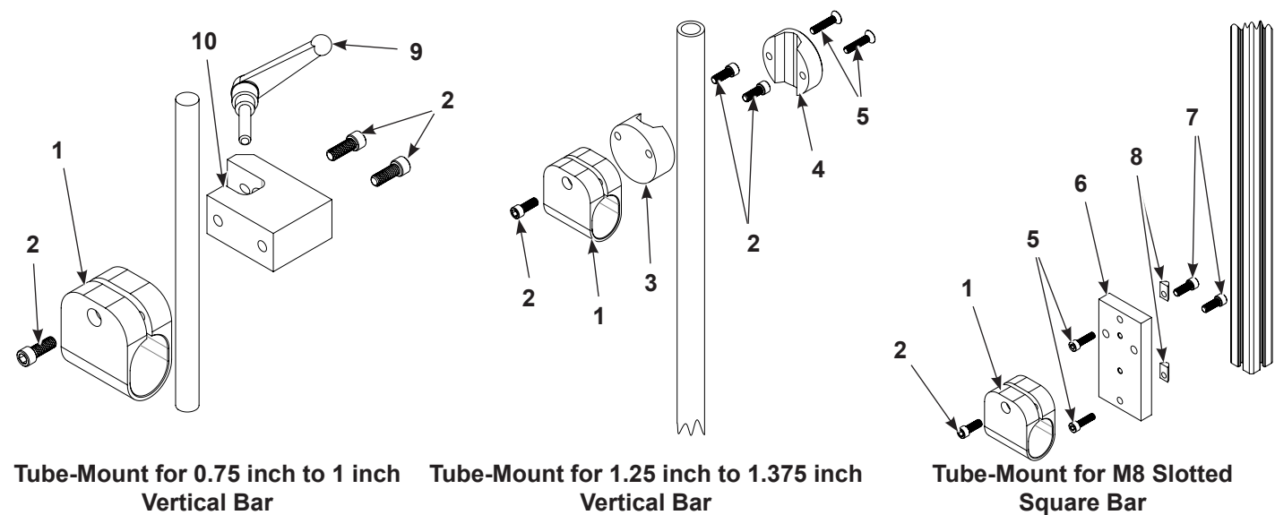
Figure 1 Spray Gun Mounts for Tube-Mount Guns
