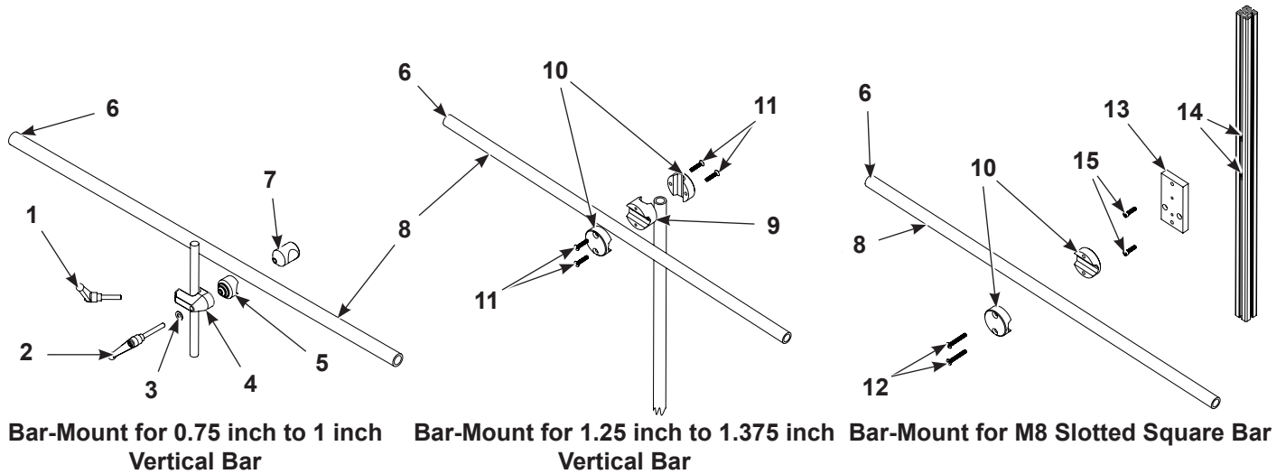
Figure 2 Spray Gun Mounts for Bar-Mount Guns
