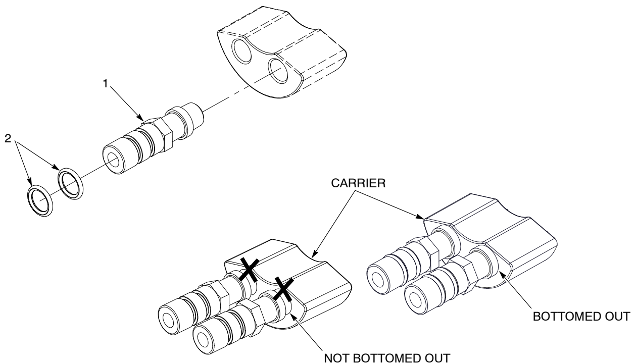
Figure 1 Quick Color Change Nozzle
