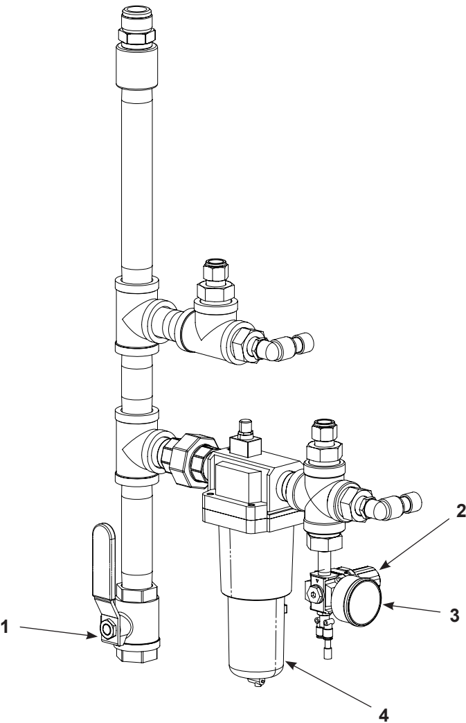
Figure 15 Air Header Assembly. View Depicts Configuration for Latch-Side Installation, Without Feed Center
