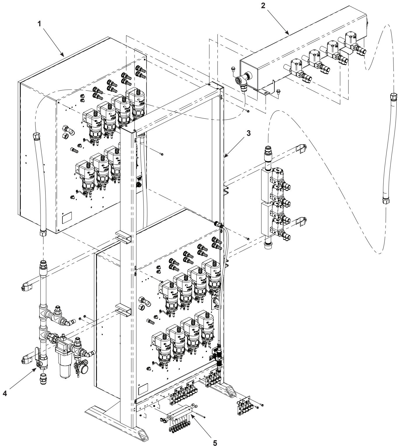
Figure 2 View Depicts a Fully Populated Stand, Configured for Use Without a Feed Center, With the Air Header Installed on the Latch Side of the Pump Cabinet
