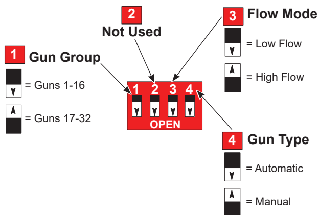
Figure 5 SW2 Settings
