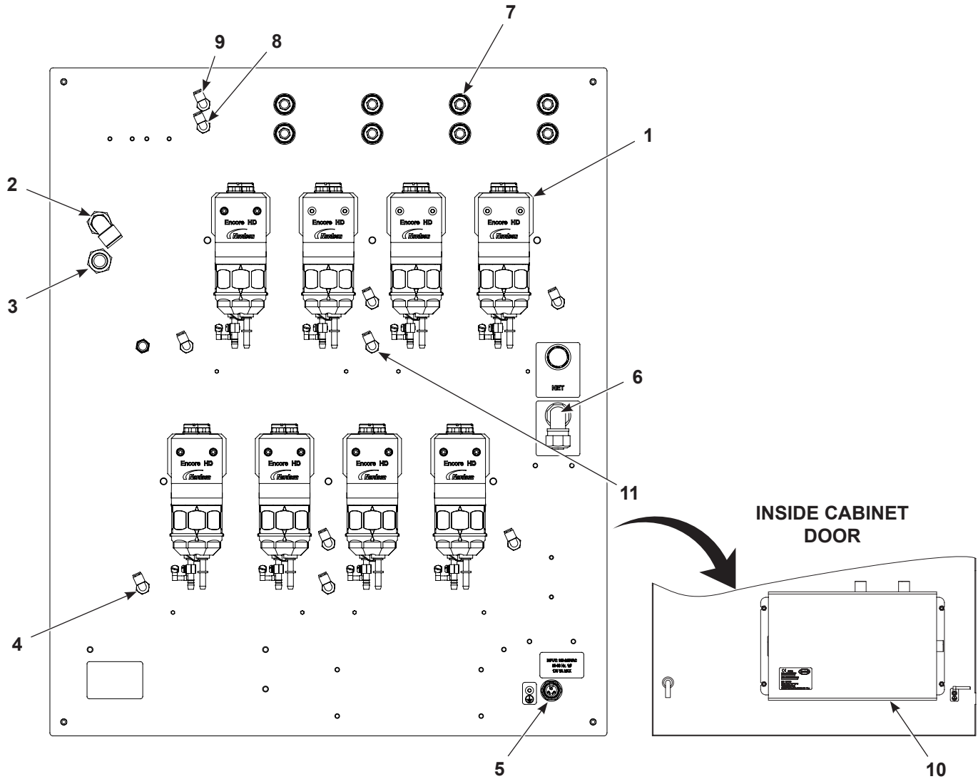
Figure 3 External Pump Panel Components (Eight-Pump Panel Shown)
