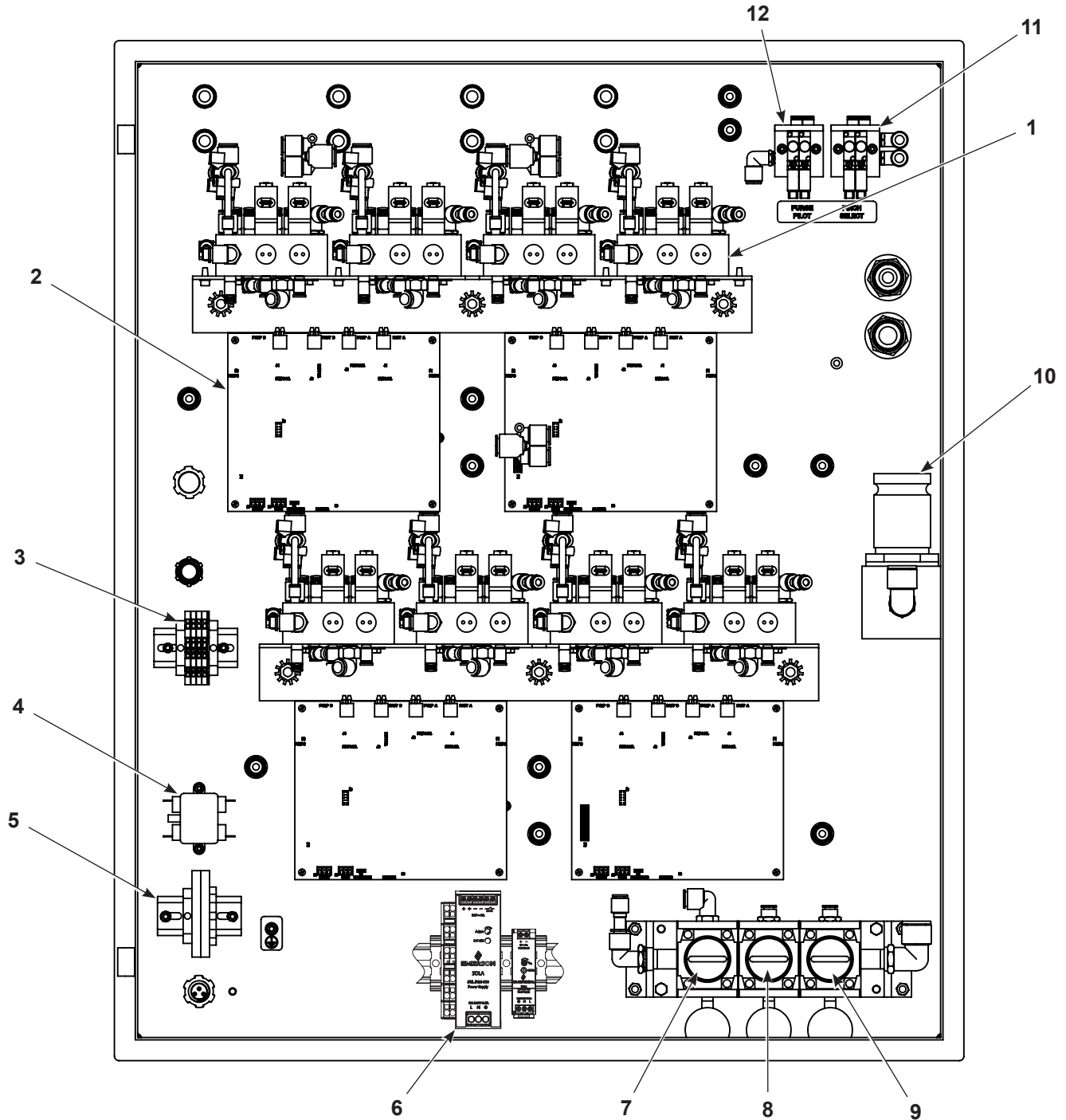
Figure 4 Internal Pump Panel Components (Eight-Pump Panel Shown)
