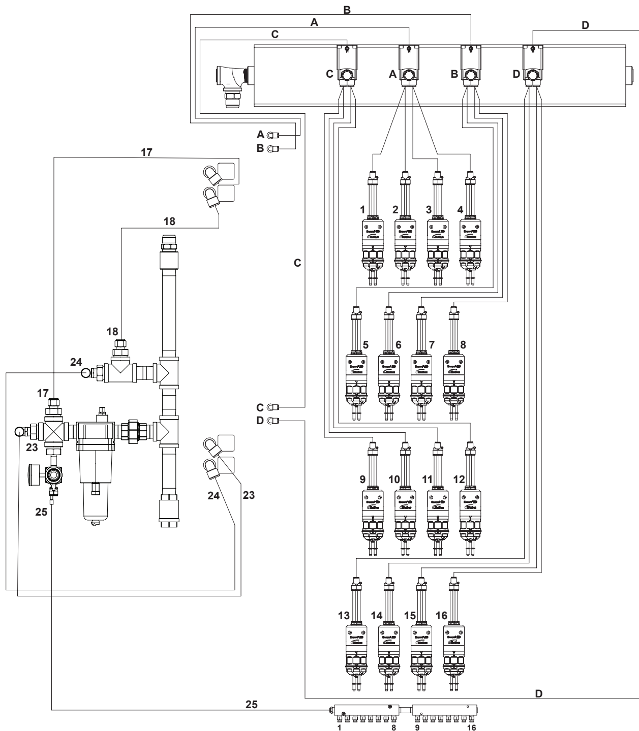
Figure 7 Pump Panel External Pneumatic Diagram (Two Eight-Pump Panels Shown)
