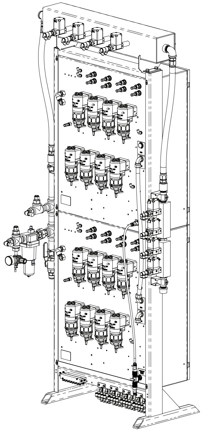
Figure 1 Encore Automatic System HD Standalone Pump Stand (Two Eight-Pump Panels are Shown)
