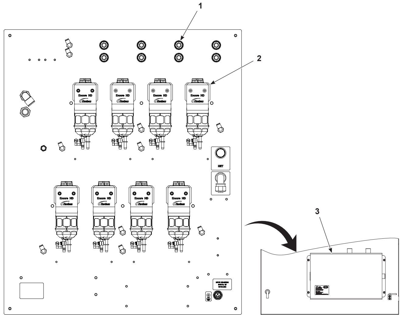
Figure 13 External Pump Panel Replacement Parts (Eight-Pump Panel Shown)
