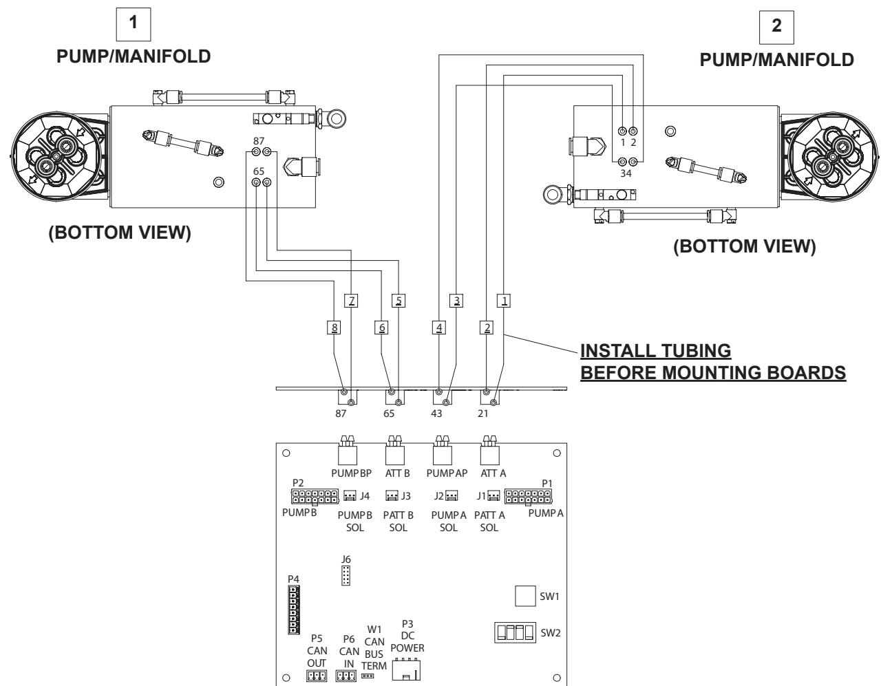
Figure 9 Pump Panel Pneumatic Diagram – Pump Manifolds to Circuit Board
