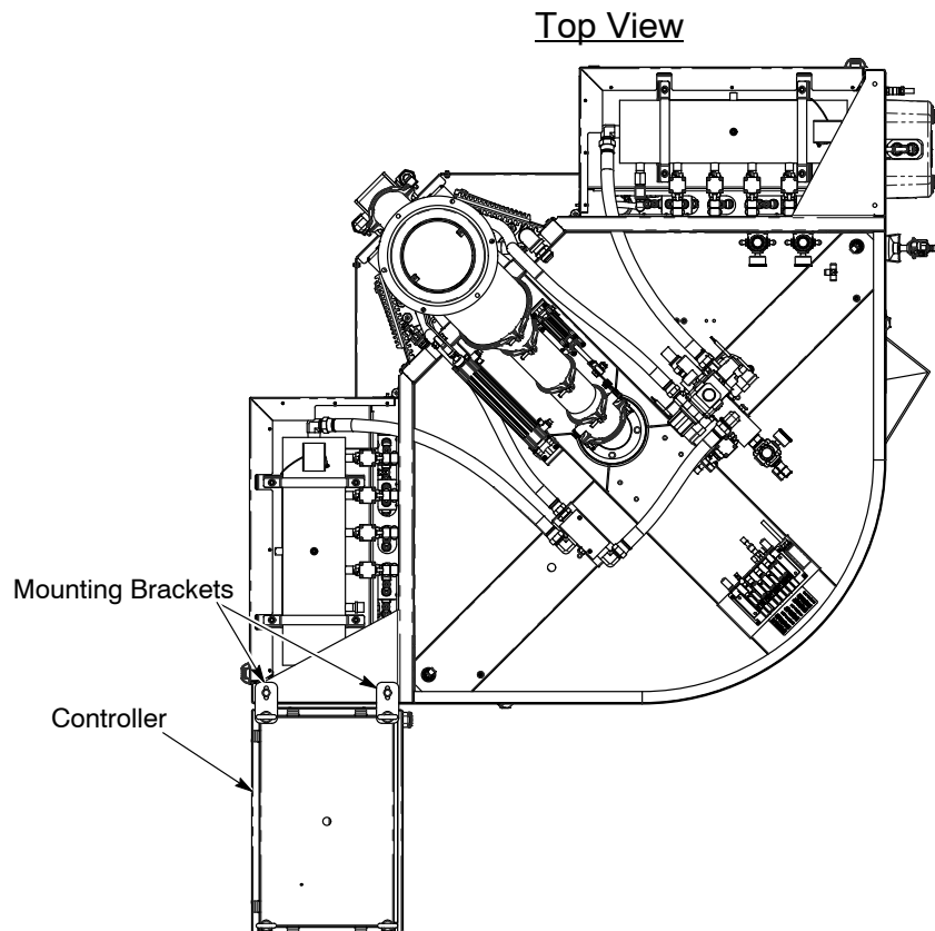
Figure 1 Mounting Bracket Location
