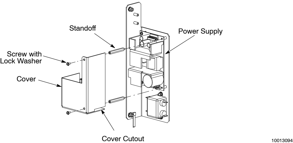
Figure 2 Installing Power Supply Cover
