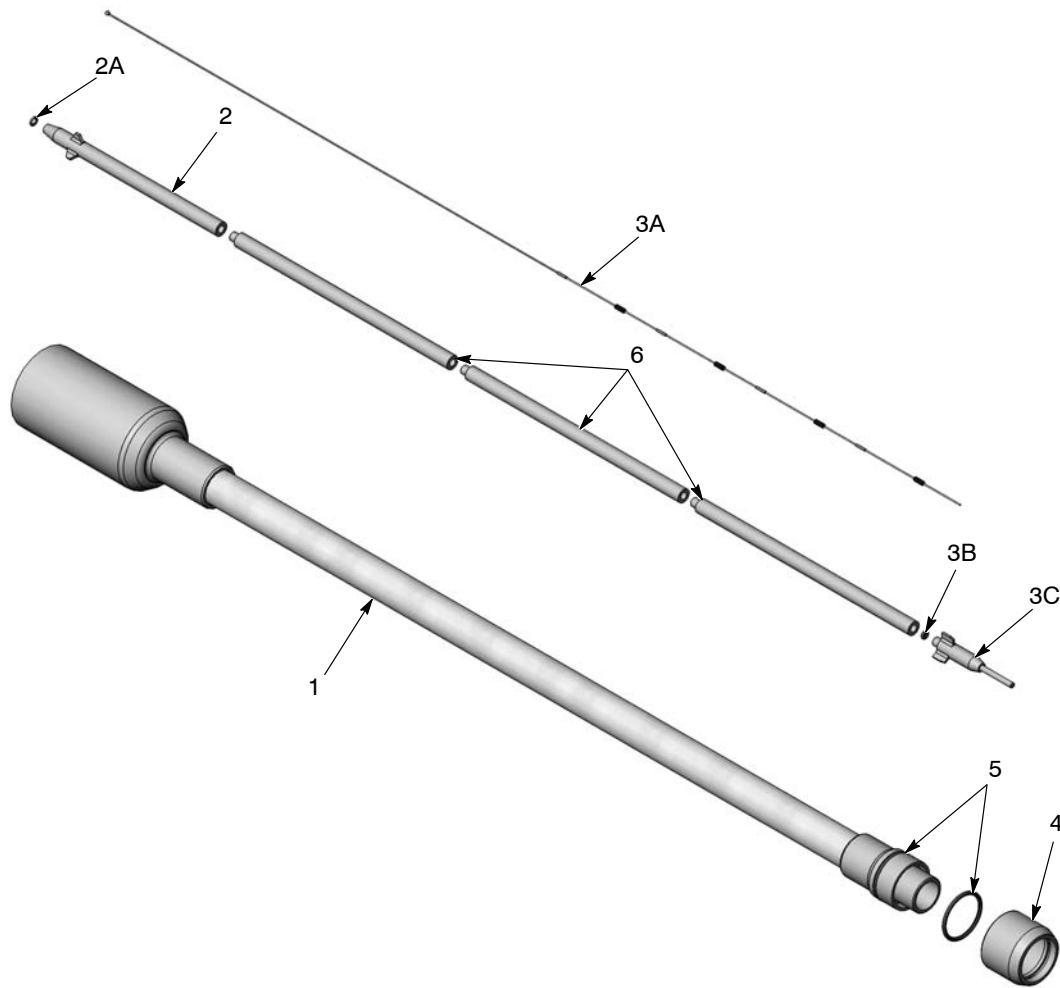
Figure 5 600-mm Lance Extension Parts
