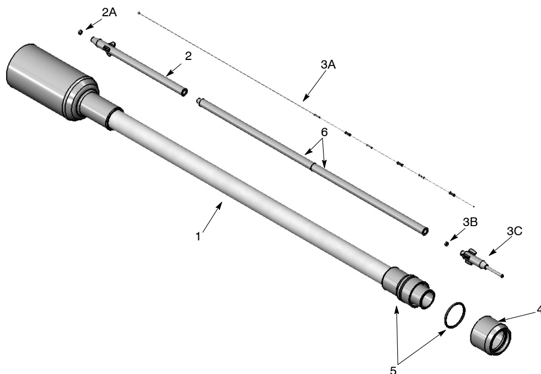
Figure 4 450-mm Lance Extension Parts
