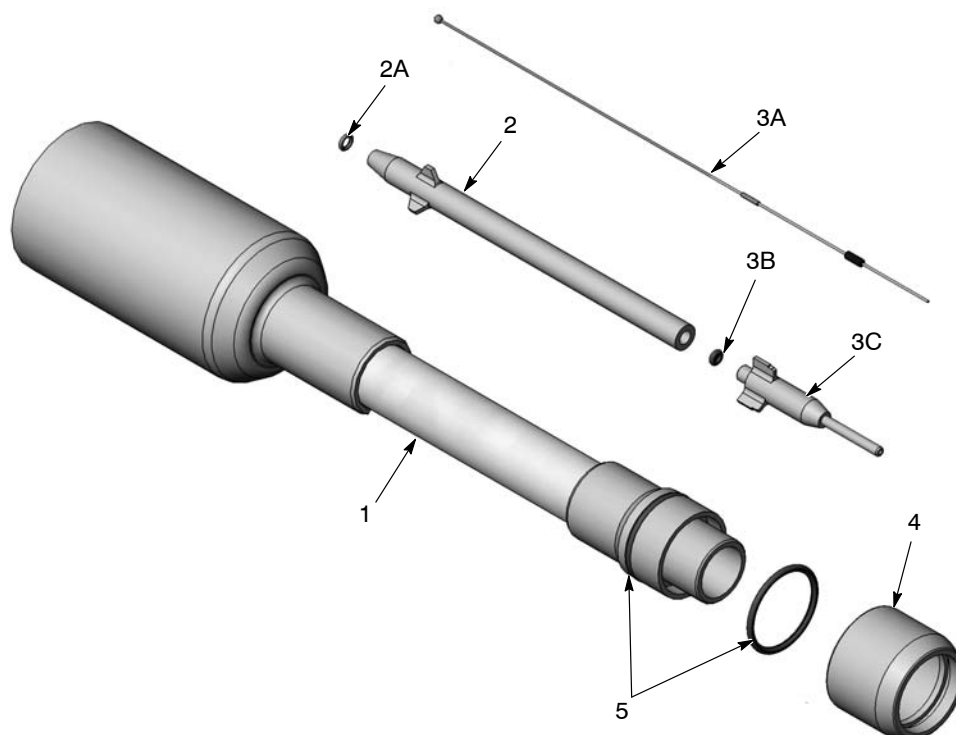
Figure 2 150-mm Lance Extension Parts
