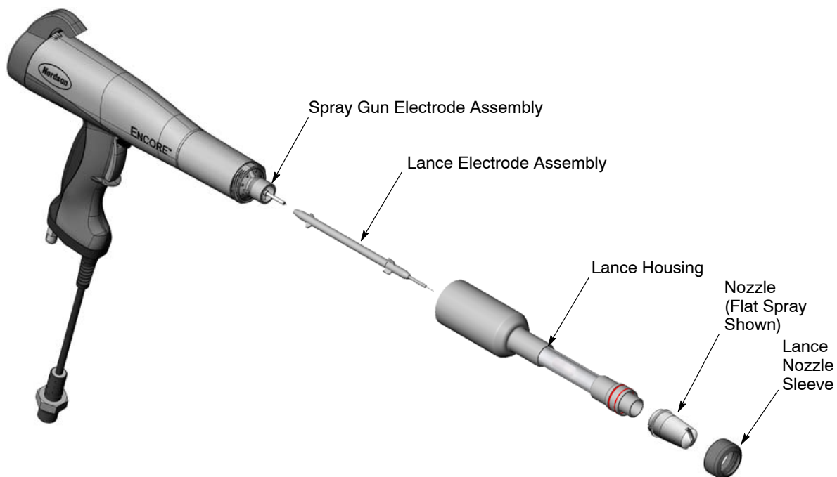
Figure 1 Lance Installation
