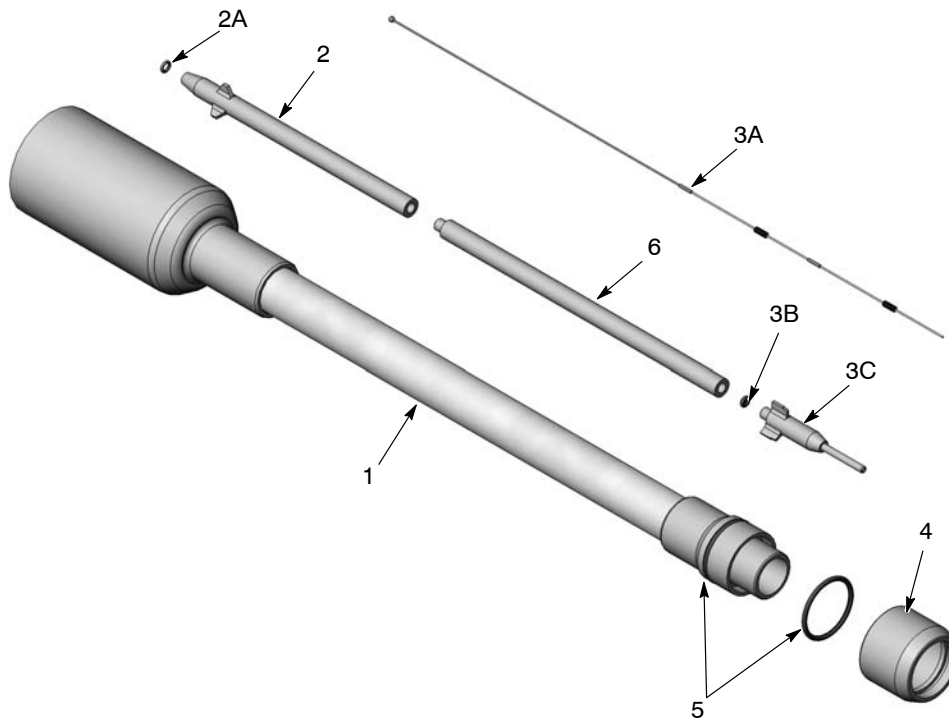
Figure 3 300-mm Lance Extension Parts
