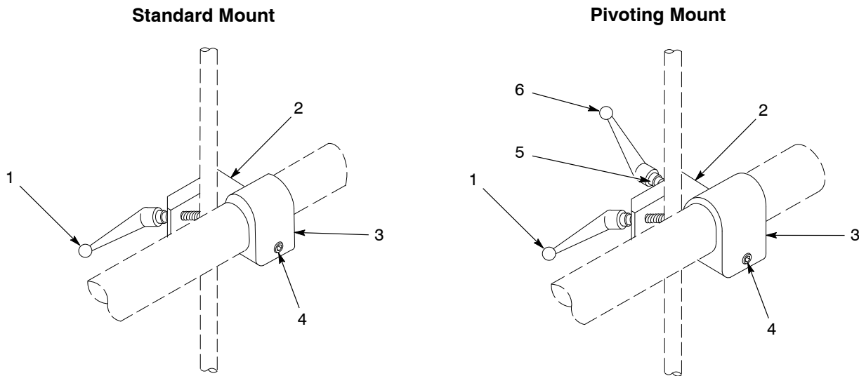
Figure 1 Gun Bar Mounts for Tube-Mount Guns
