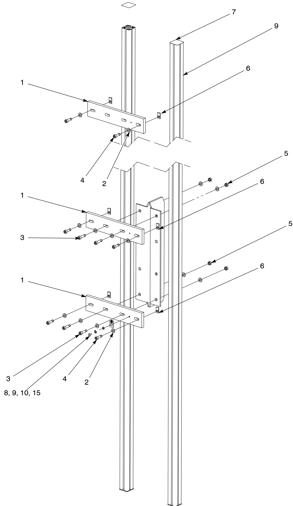
Figure 9 Three-Meter Bar Gun Support Kit
