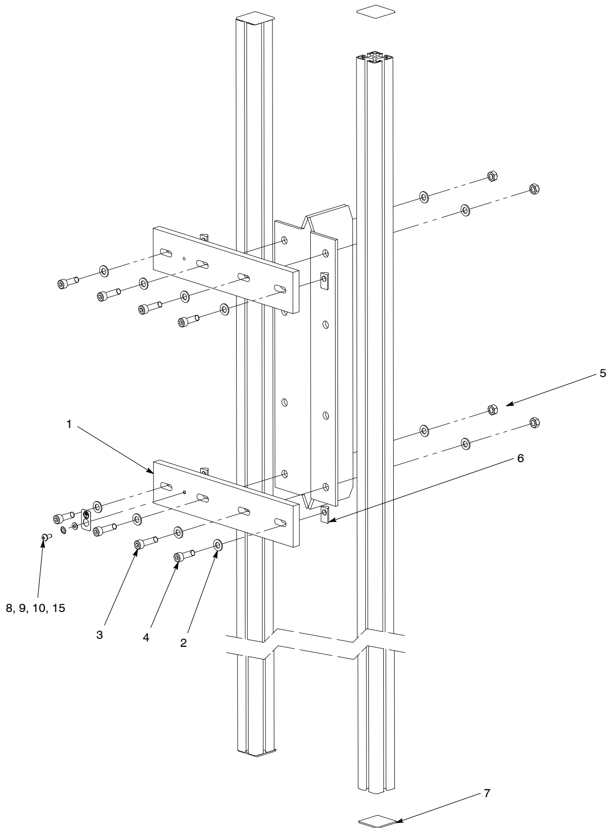
Figure 7 Dual-Bar 1 m and 2 m Gun Support Kit
