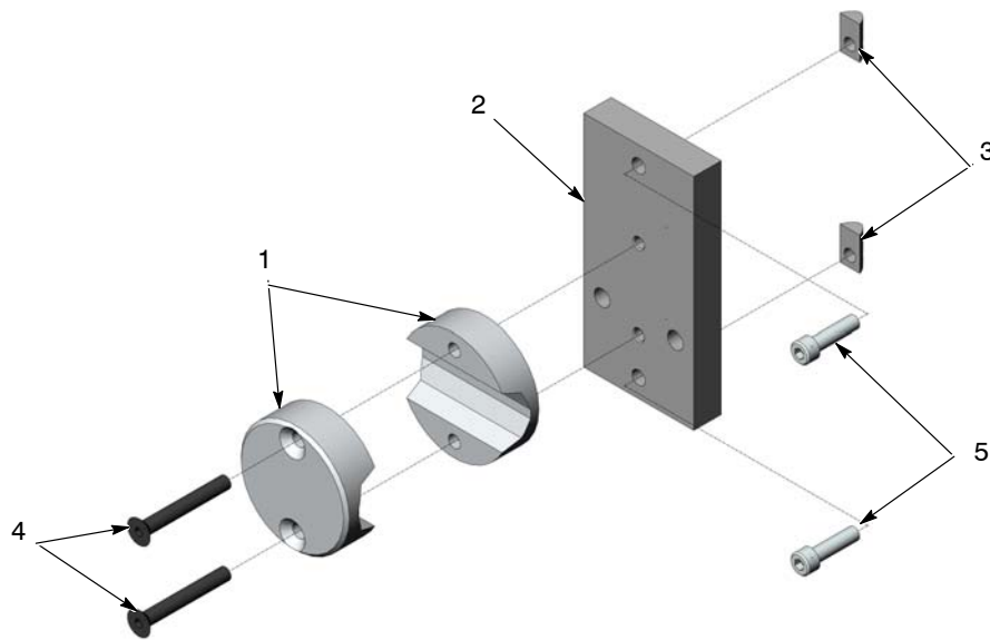
Figure 11 Vertical Bar Gun Mount for Sure Coat and Encore Tube-Mount Guns
