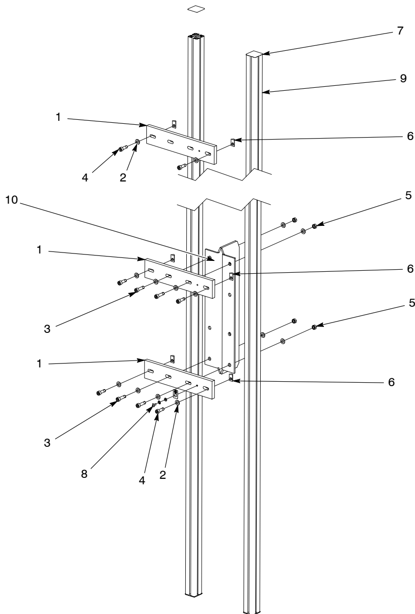
Figure 5 Three-Meter Gun Support Assembly
