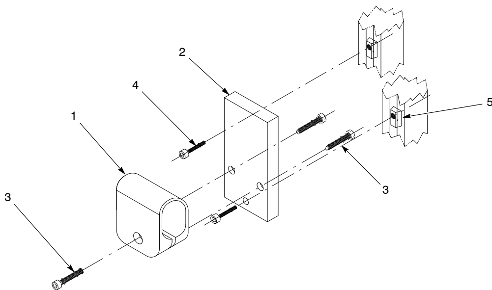
Figure 10 Vertical Bar Gun Mount for Sure Coat and Encore Tube-Mount Guns
