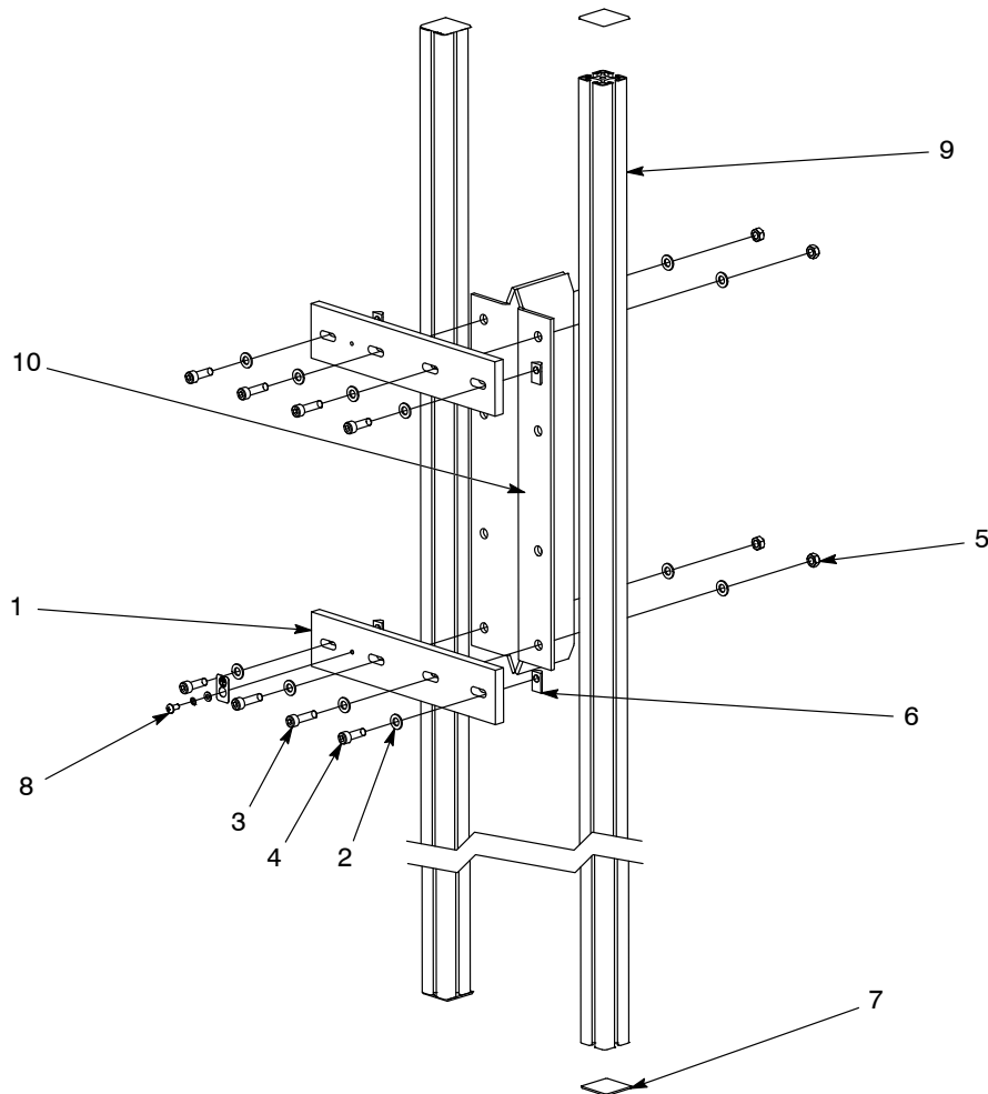
Figure 3 Dual-Bar Gun Support Assembly
