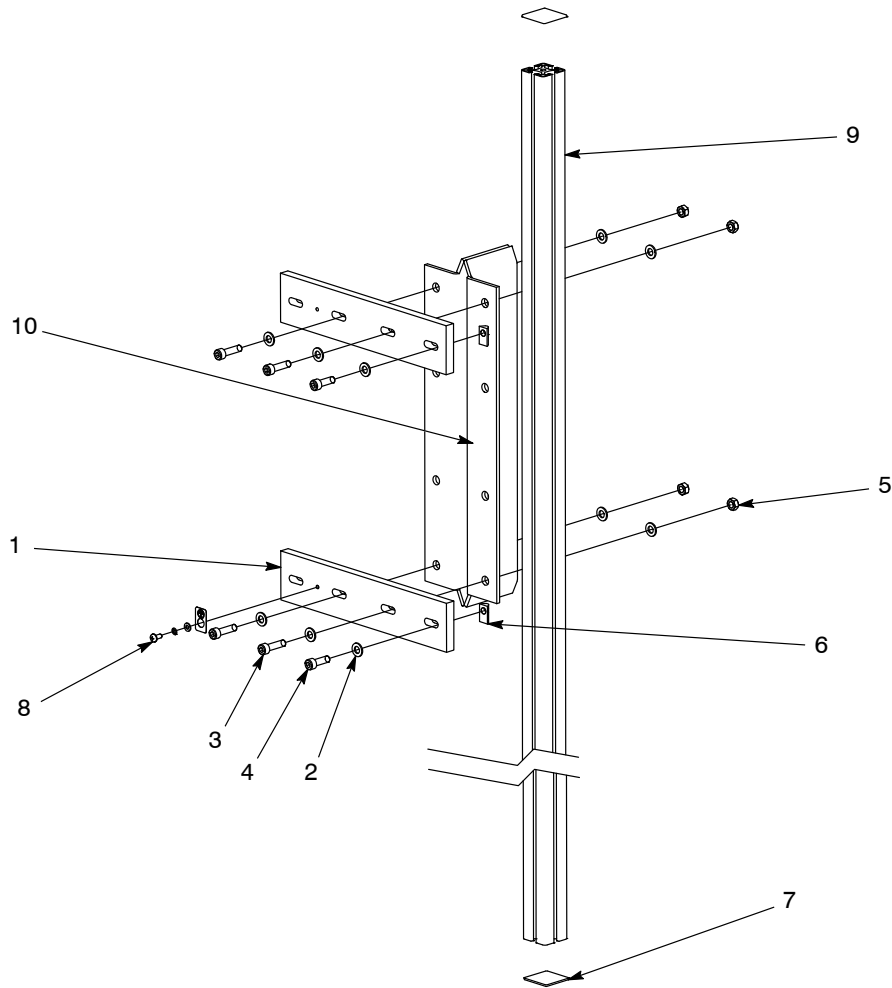
Figure 4 Single Bar Gun Support Assembly
