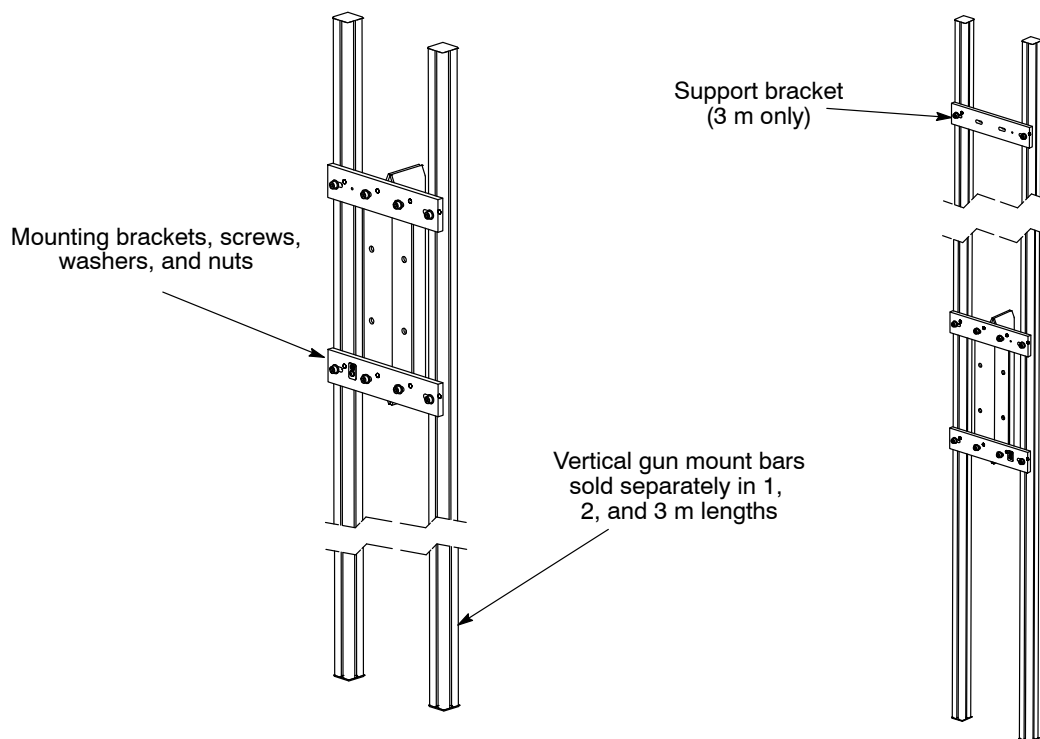
Figure 2 Dual Vertical Extruded Support Kit
