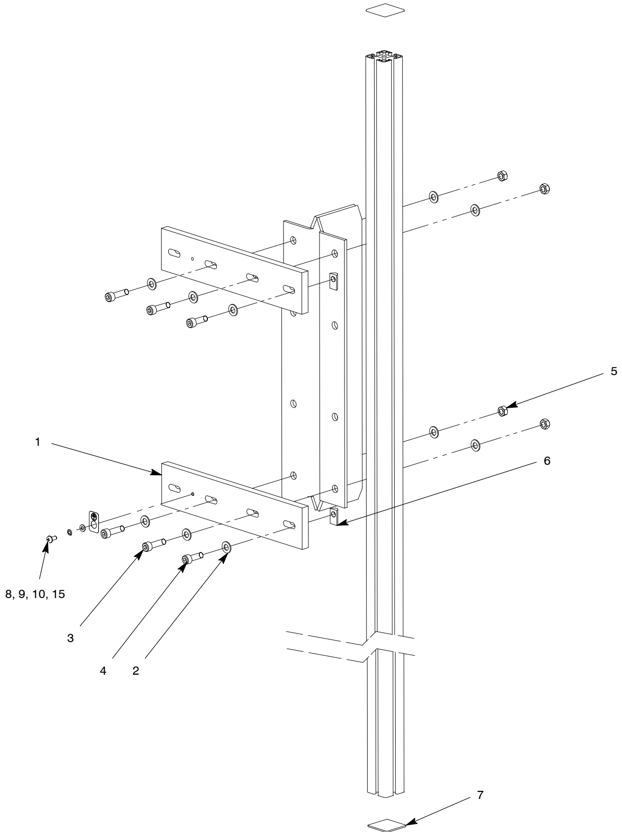
Figure 8 Single-Bar Gun Support Kit
