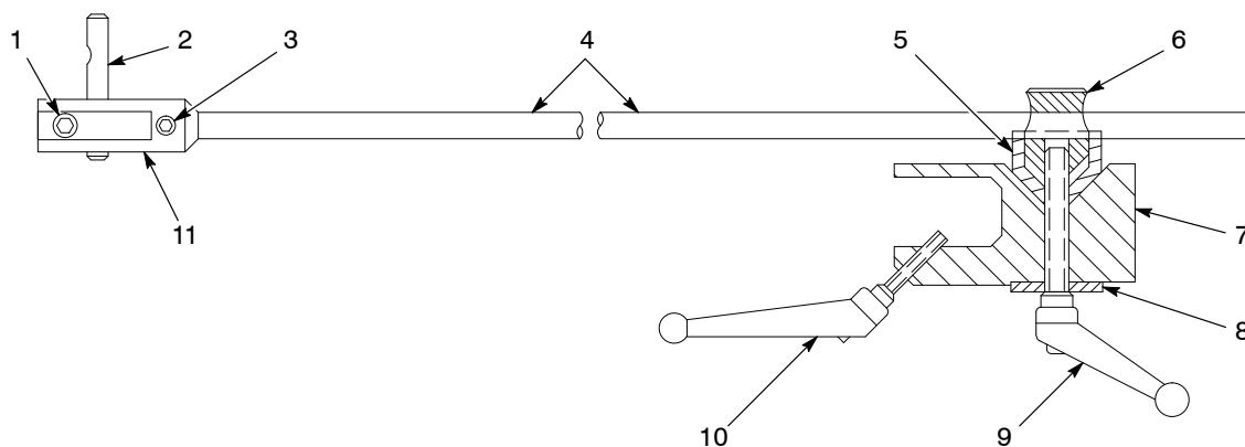
Figure 1 Gun Mounting Bar
