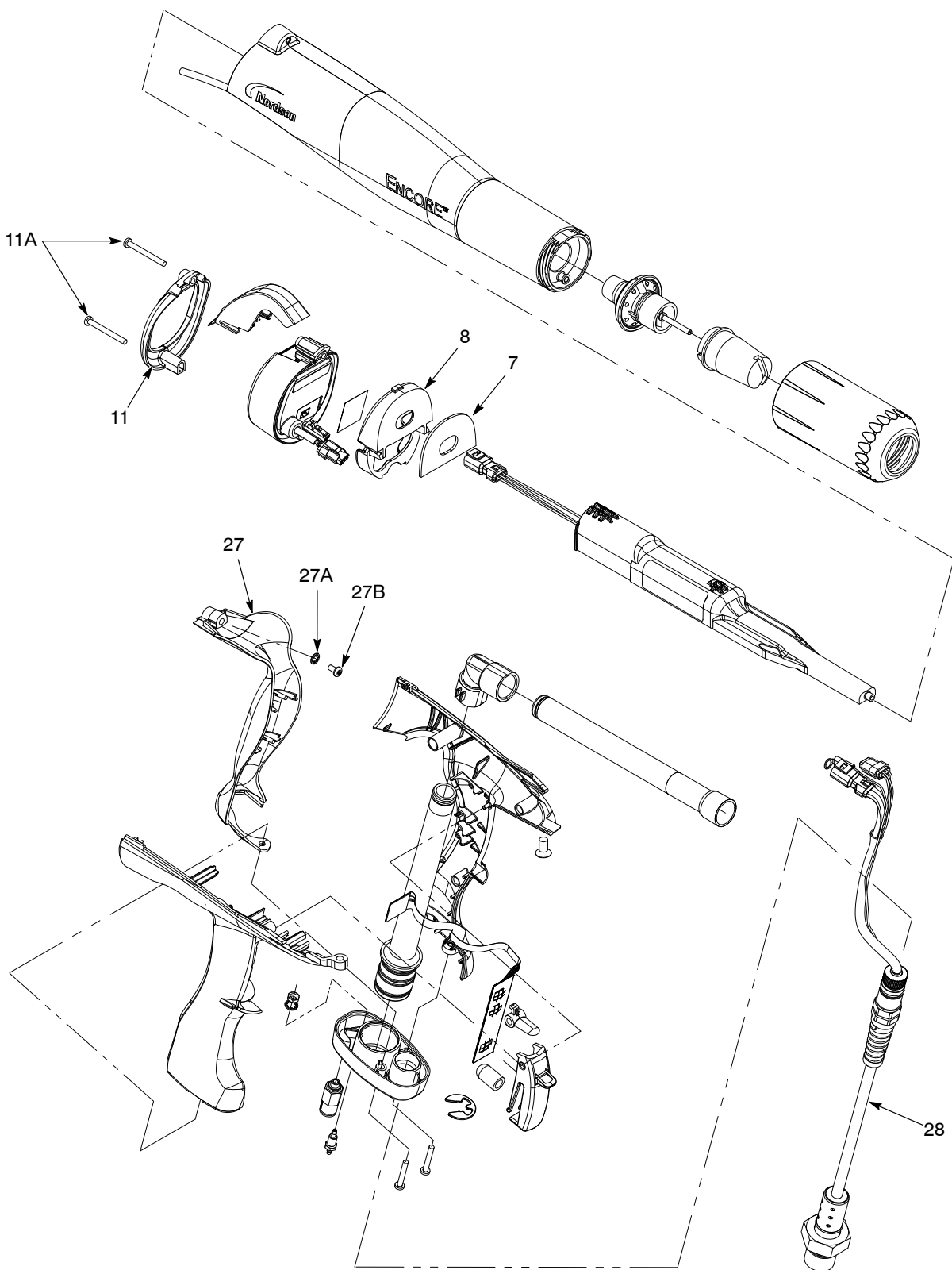
Figure 11 Kit Parts
