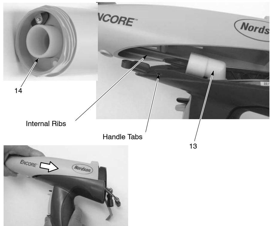
Figure 10 Outlet Tube, Elbow, and Gun Body Installation
