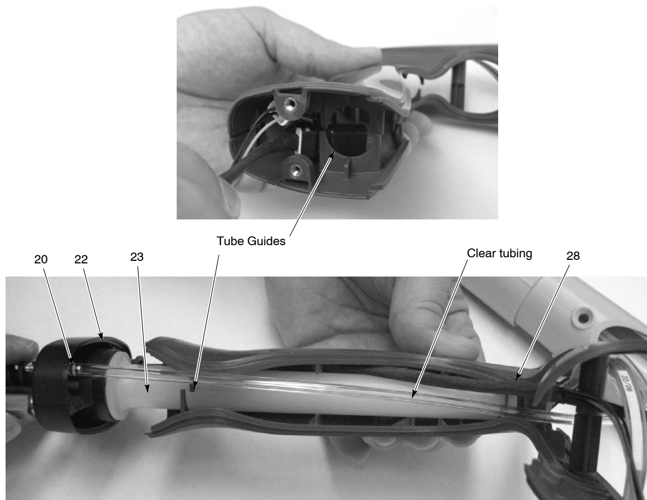
Figure 6 Assembling Handle
