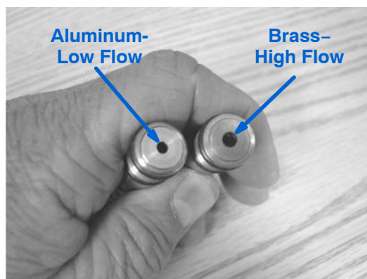
Figure 3 Low Flow and High Flow Restrictor Plates
