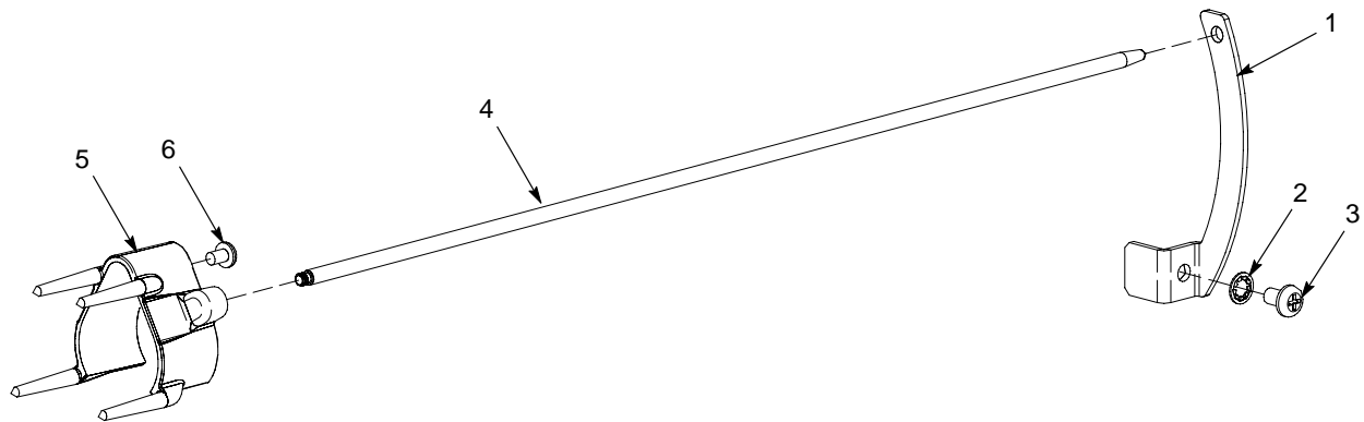
Figure 4 Bar Mount Kit Parts
