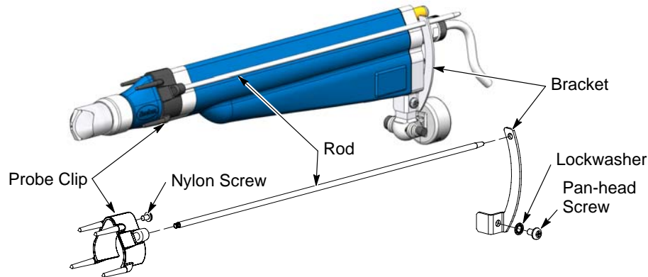
Figure 2 Bar Mount Gun Kit Installation
