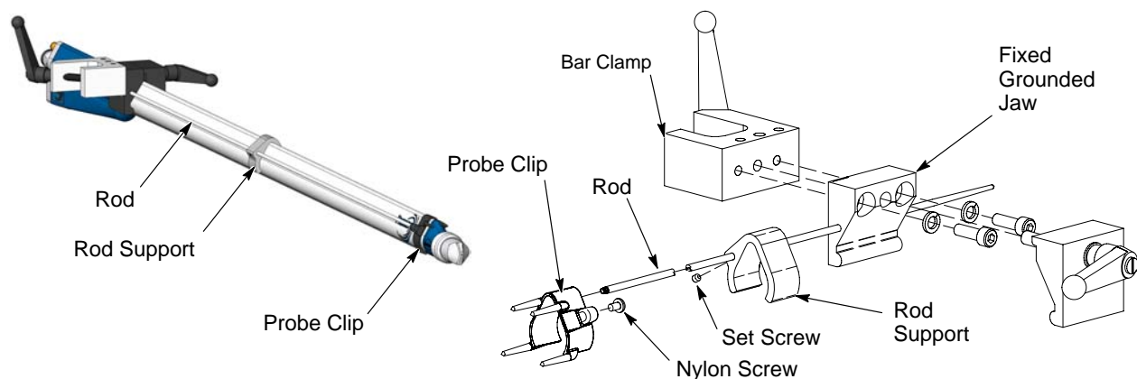
Figure 1 Tube Mount Gun Kit Installation
