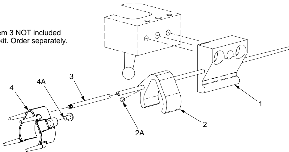
Figure 3 Tube Mount Kit Parts
