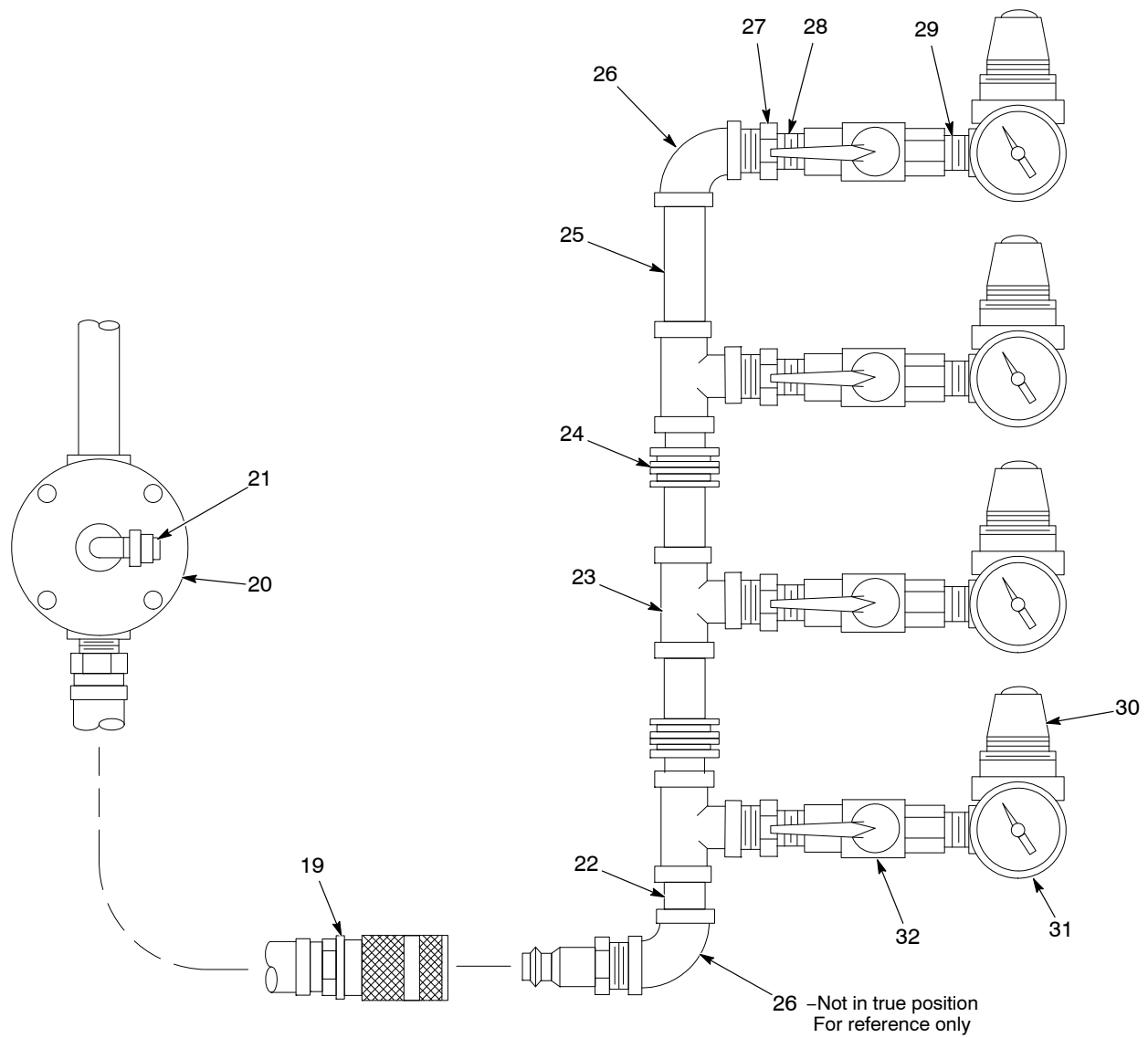
Figure 2 Dolly Parts (2 of 2)
