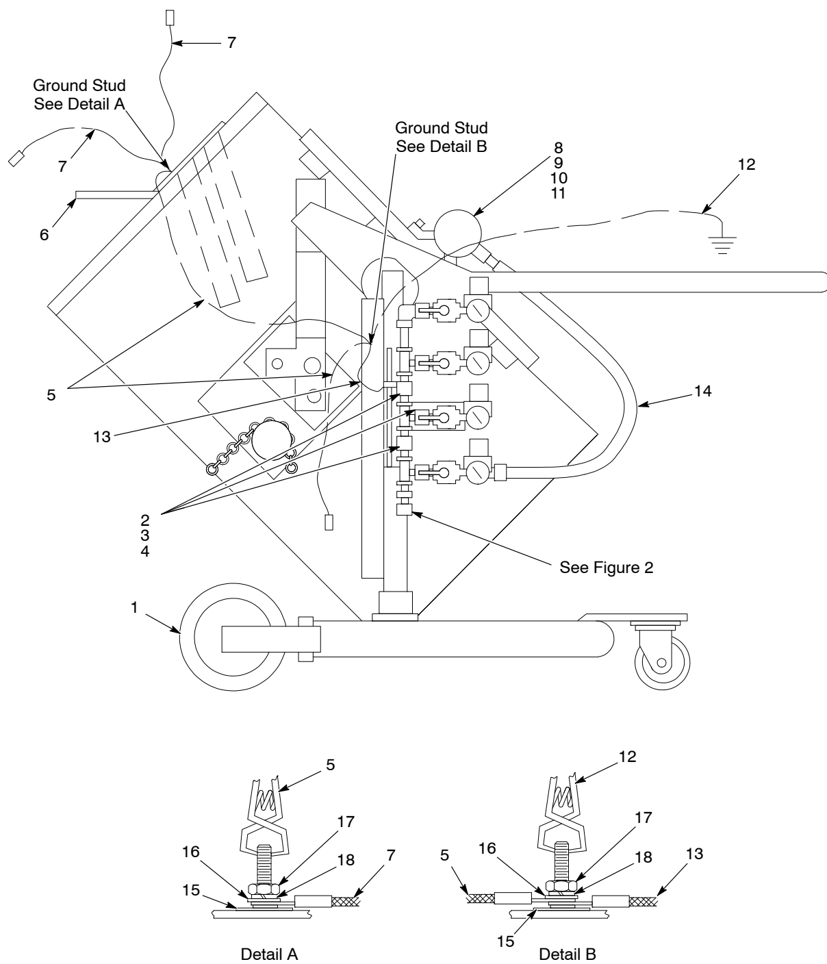
Figure 1 Dolly Parts (1 of 2)
