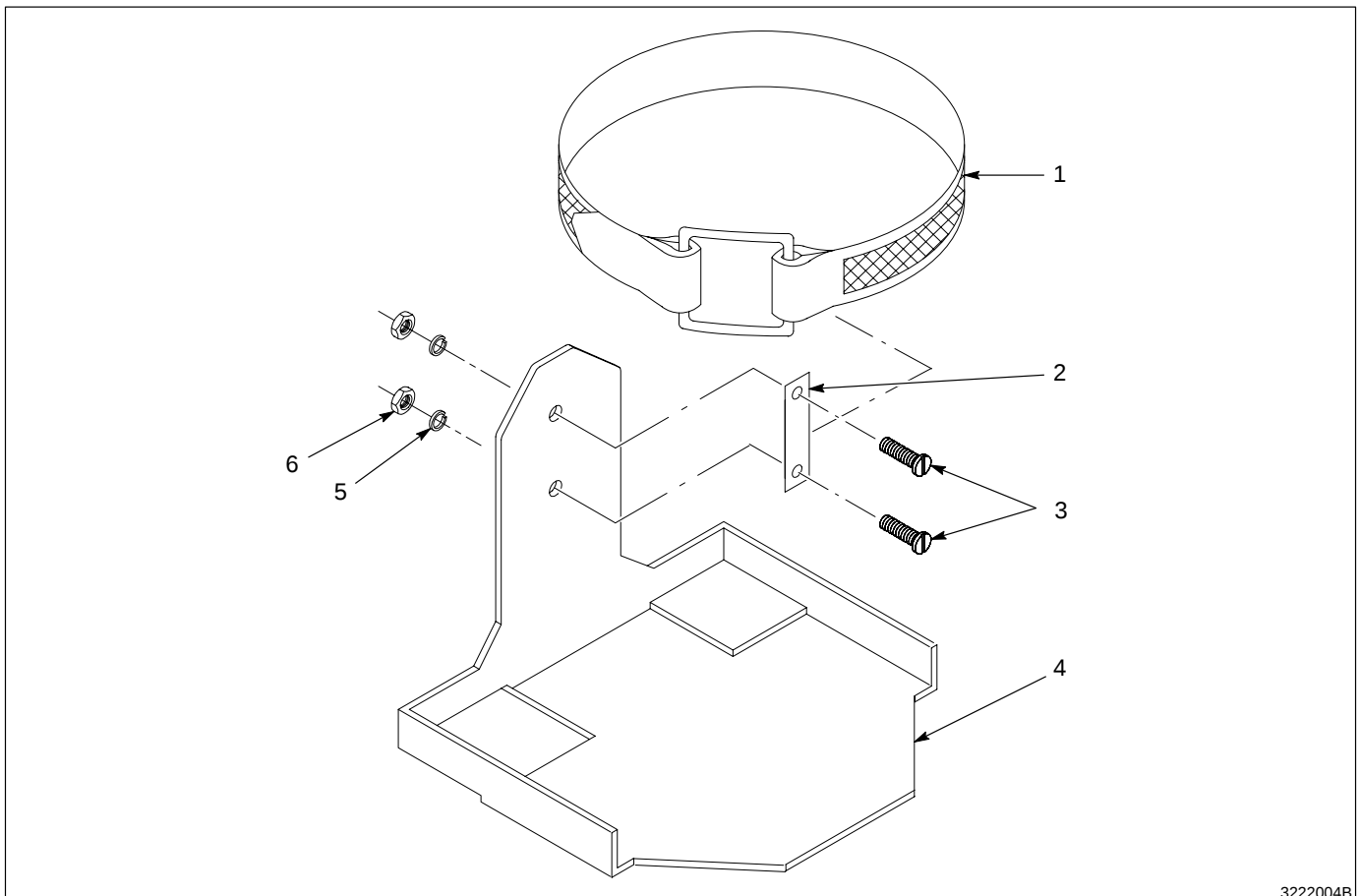
Fig. 1 Mounting Kit
