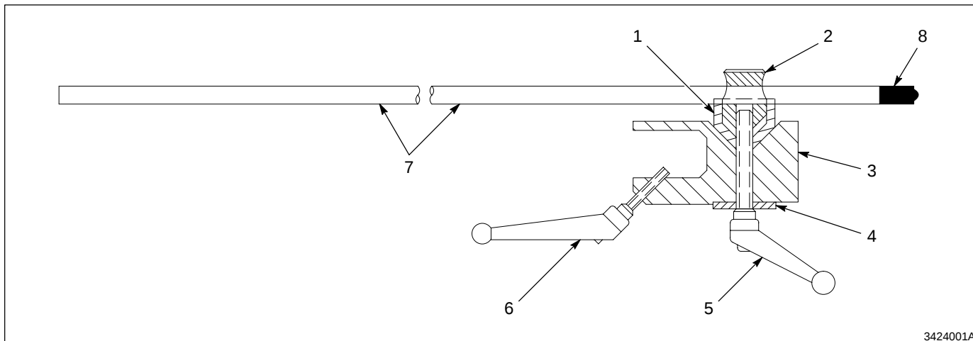
Fig. 1 Versa-Spray Gun Mounting Bar
