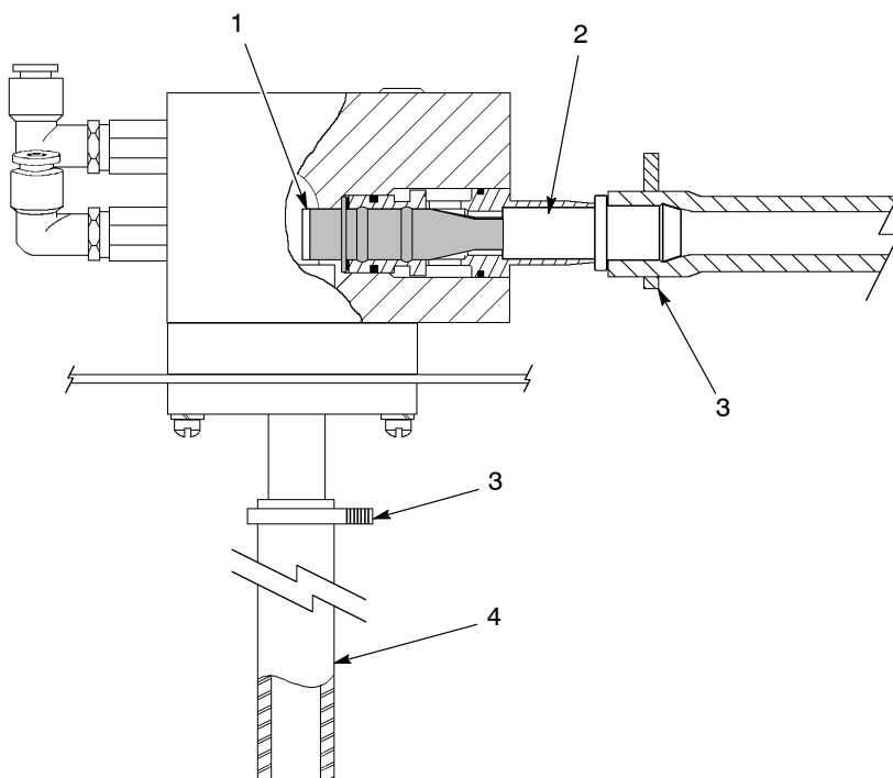
Figure 2 Low-Flow Conversion Kit 114217
