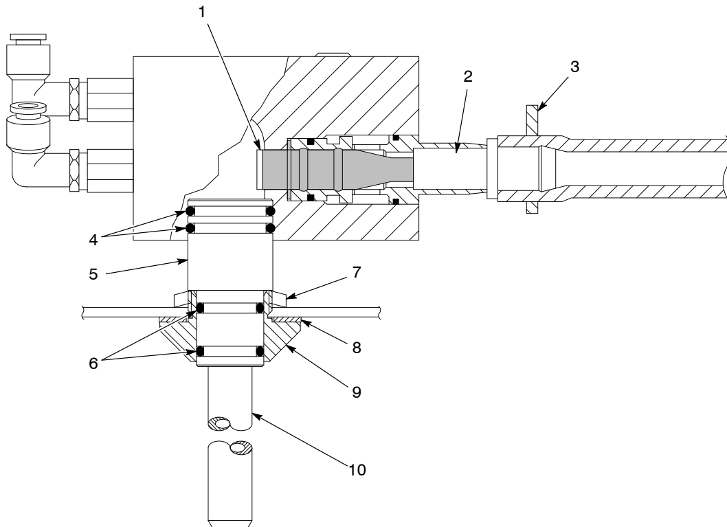
Figure 3 Conversion Kit 118743
