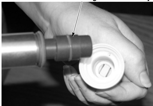
Figure 8 Nozzle Disassembly Step 2B (New Style Assembly Shown)
