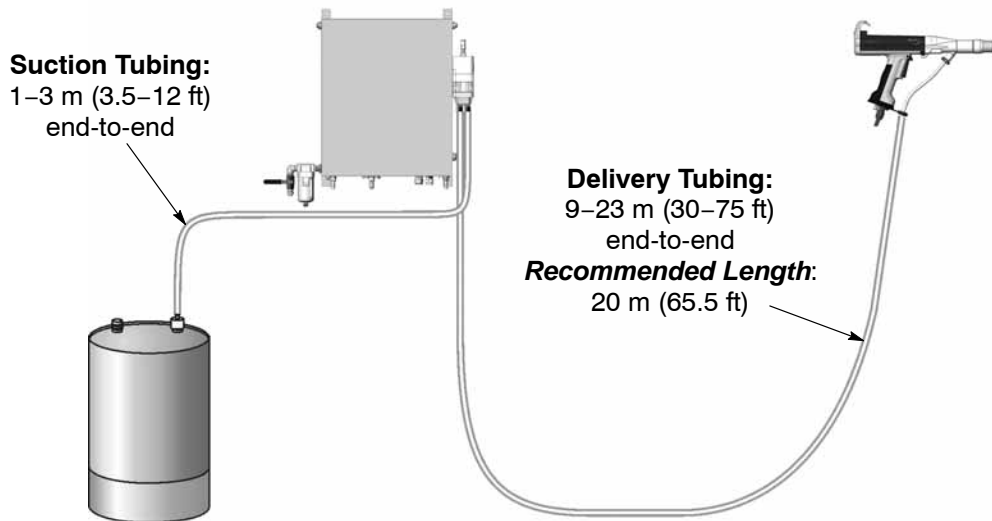
Figure 3 Determining Powder Tubing Length
