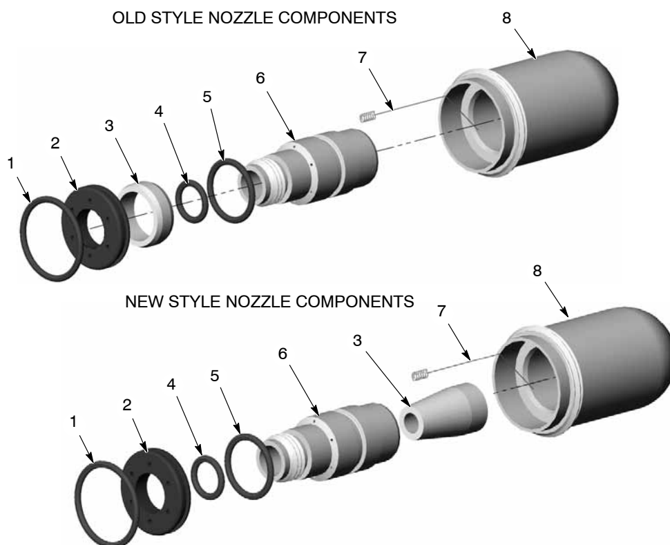
Figure 11 Internal Components of Nozzle Assemblies
