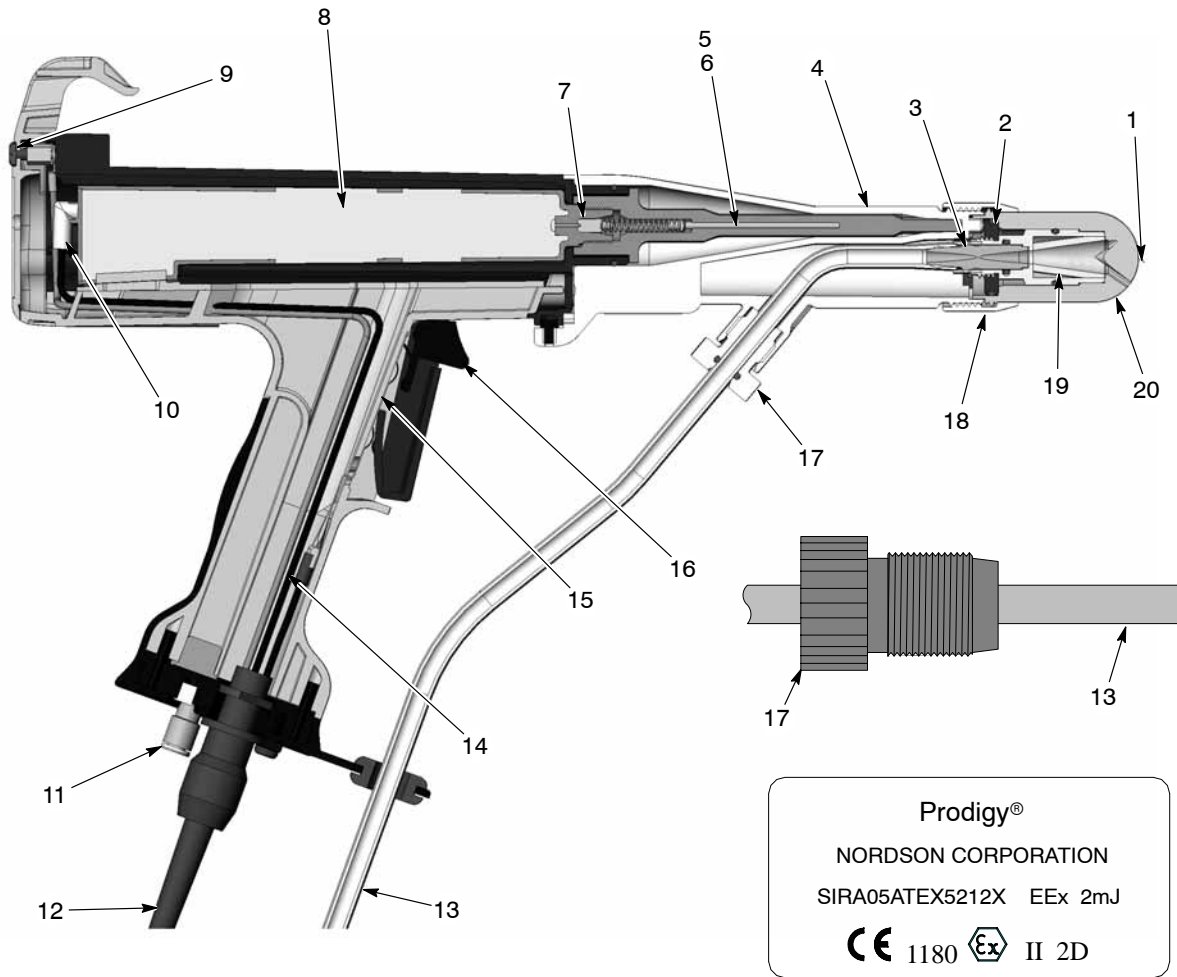
Figure 2 Spray Gun Section View
