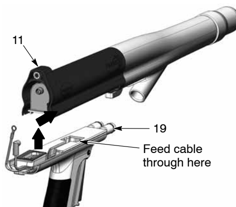
Figure 22 Separating the Gun Body from the Handle
