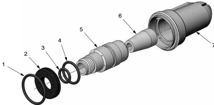
Figure 34 Flat Spray, Cross, and Pinpoint Nozzle Components
