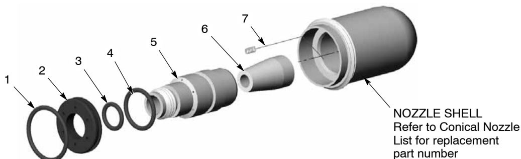
Figure 32 Conical Nozzle Components
