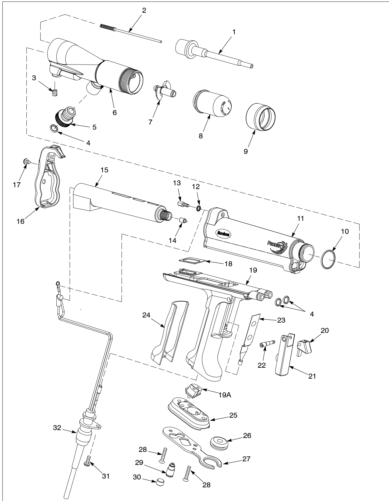
Figure 29 Prodigy Manual Spray Gun Exploded Parts Illustration
