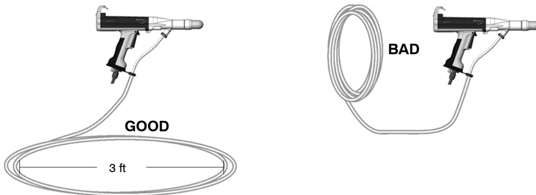
Figure 4 Coiling the Powder Tubing
