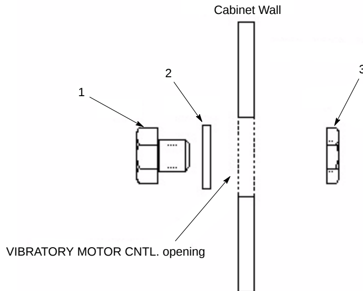
Figure 1 Vibratory Motor Control Plug Kit
