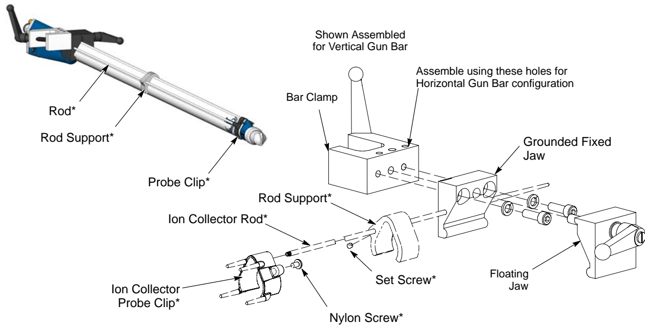
Figure 1 Tube-Mount Gun Mounting (*= Ion Collector Components)
