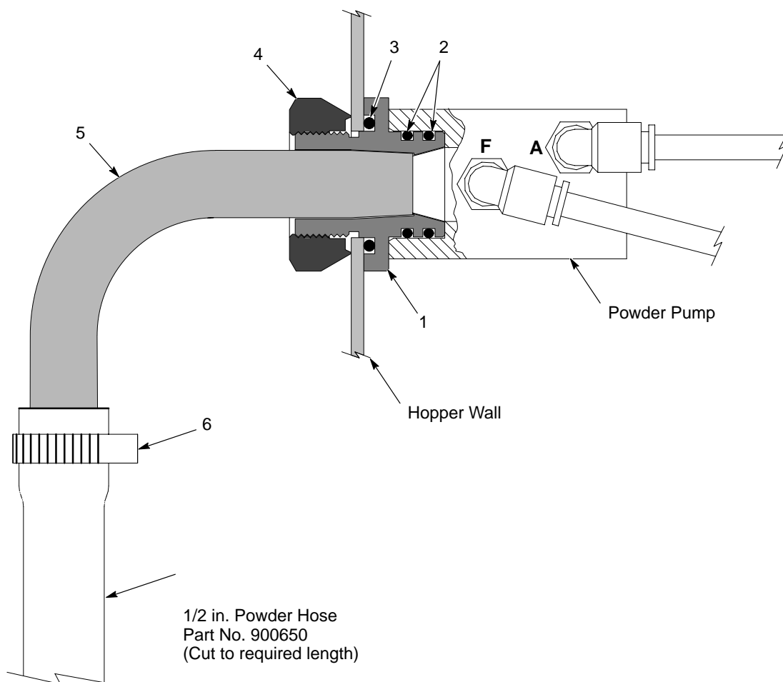
Figure 1 Side Mount Pump Mounting Kit Installation
