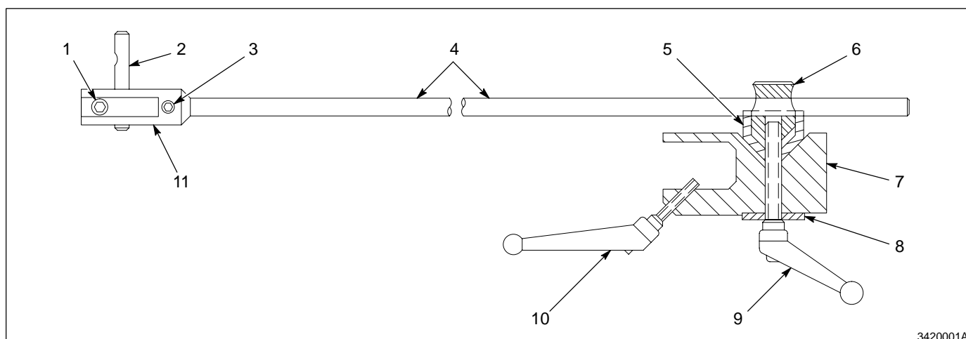
Fig. 1 Gun Mounting Bar
