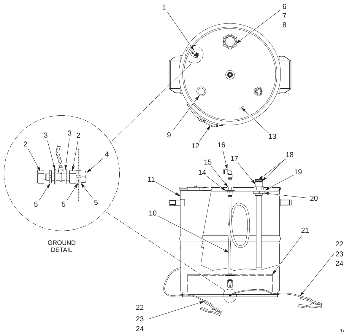
Figure 1 Econo-Coat 25-lb Powder Feed Hopper Replacement Parts
