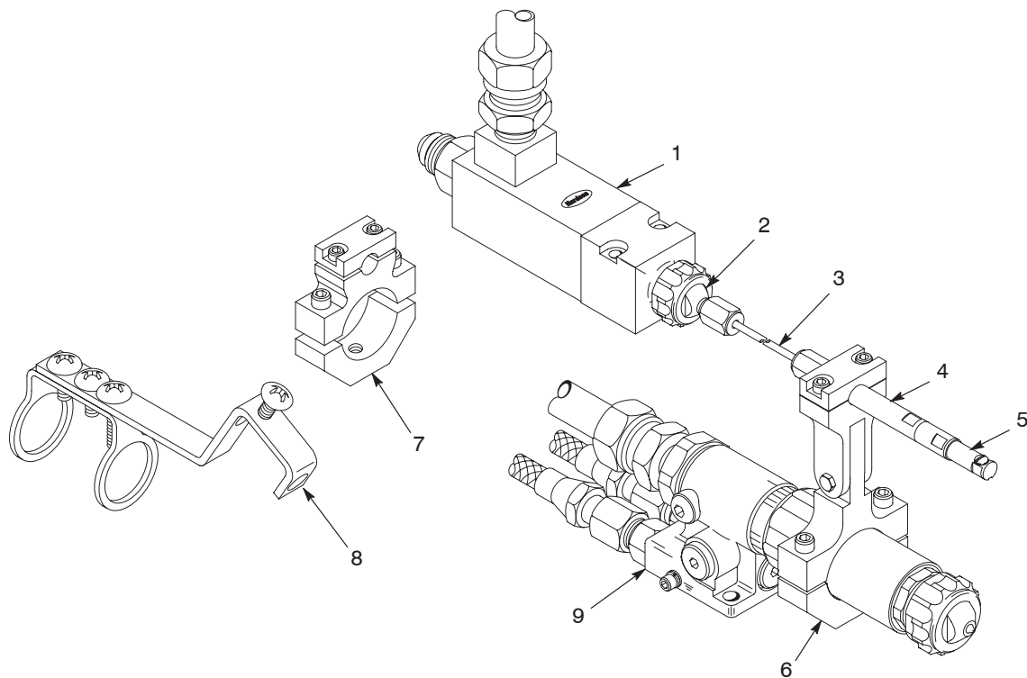
Figure 1 CleanSpray II Extension Assembly and Brackets
