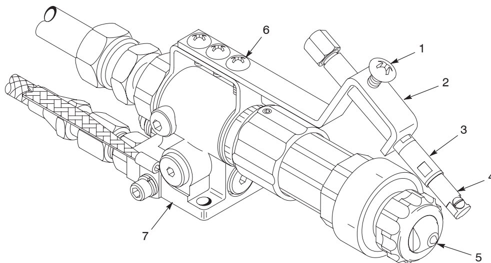
Figure 4 Bracket and Strap Assembly, Check Valve, and Nozzle Installation on MEG Gun
