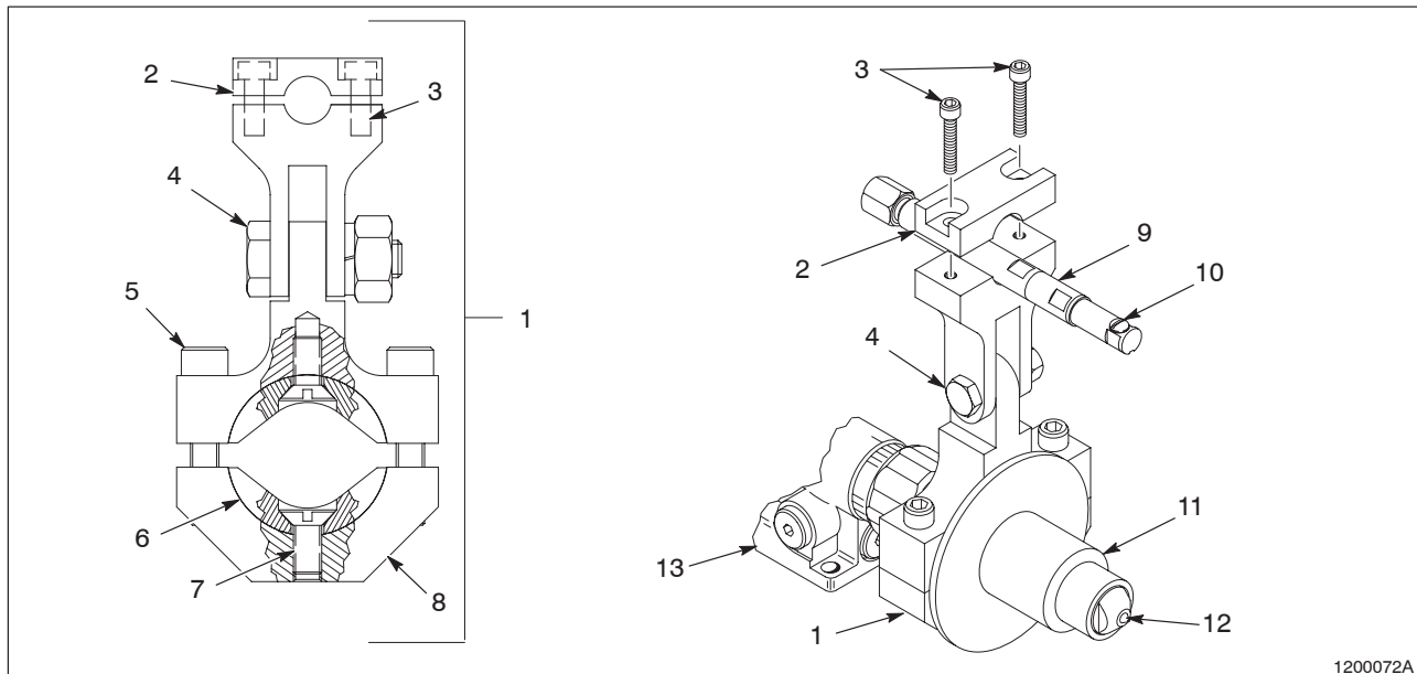
Figure 2 Adjustable Bracket, Check Valve, and Nozzle Installation (MEG Gun Installation Shown)
