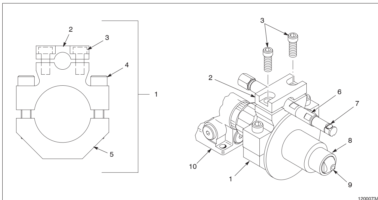
Figure 3 Fixed Mounting Bracket, Check Valve, and Nozzle Installation (MEG Gun Installation Shown)
