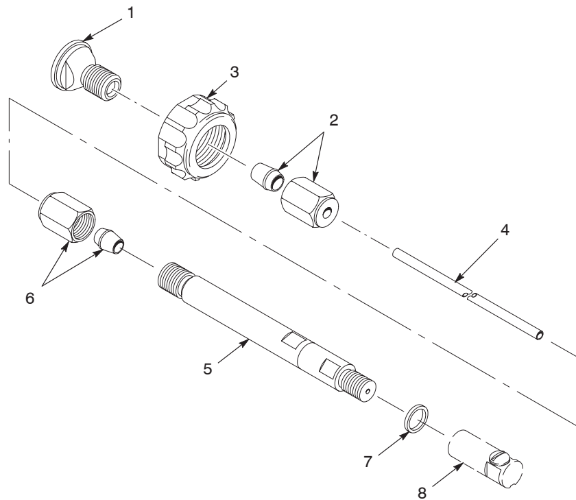
Figure 6 Extension Assembly Parts
