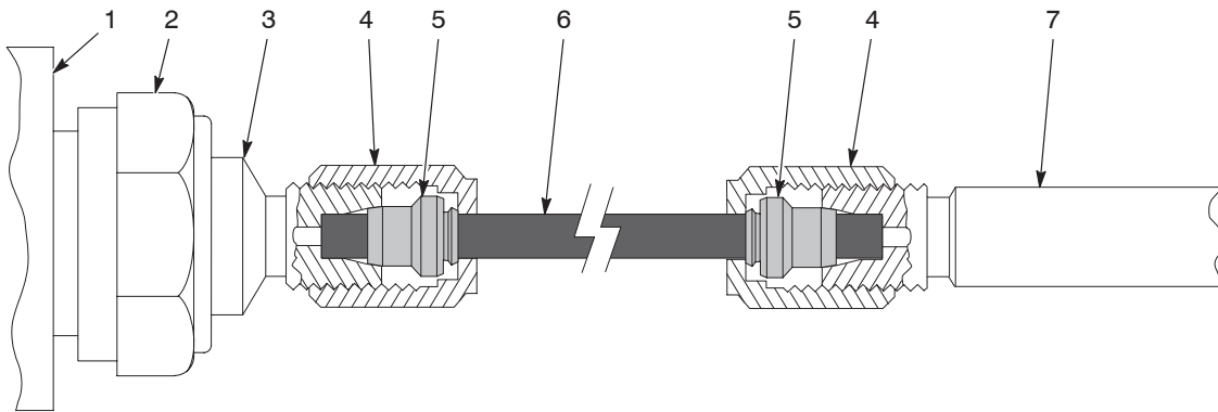
Figure 5 Tube Installation
