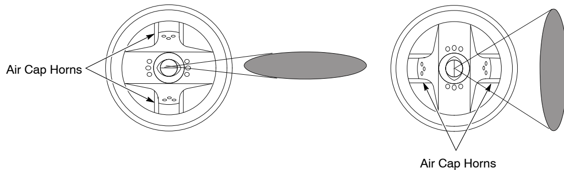
Figure 2 Air Cap Position Determines Fan Pattern Orientation
