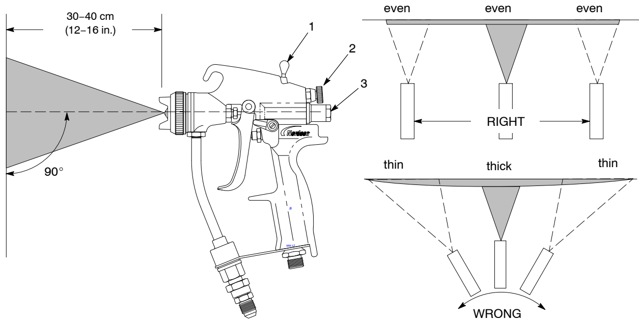
Figure 3 Proper Gun Orientation and Adjustments While Spraying
