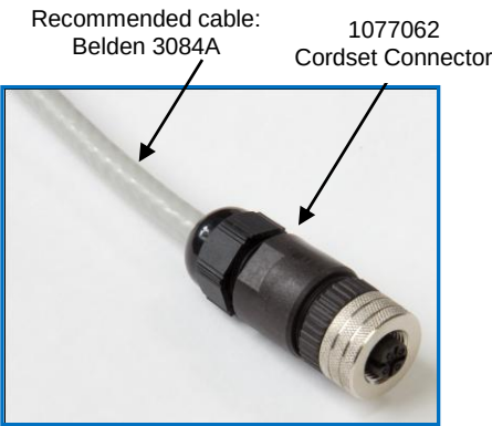
1602475 Cable Assembly w/Connector, 3 m
