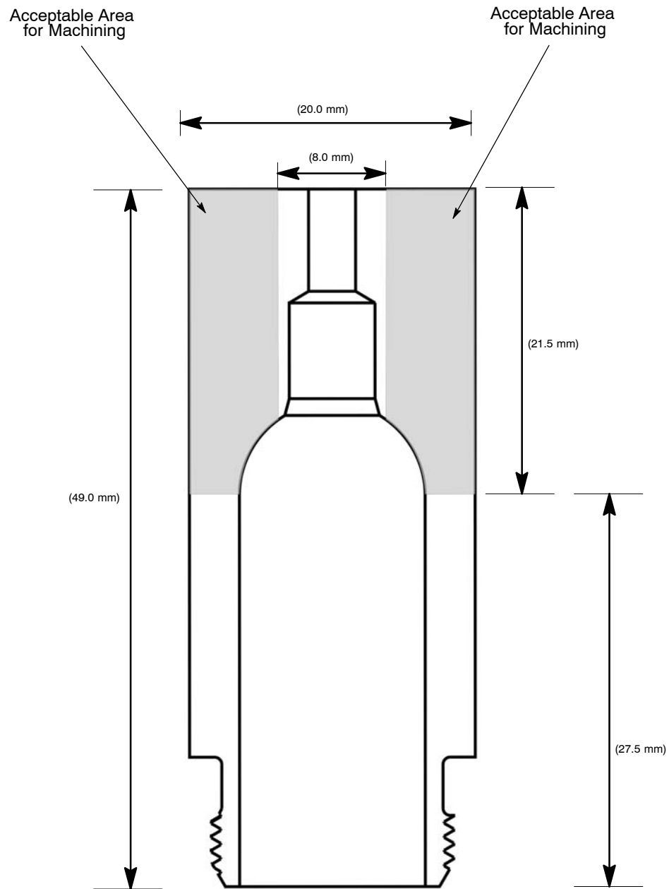
Figure 2 Blank Nozzle with Acceptable Machining Zones
