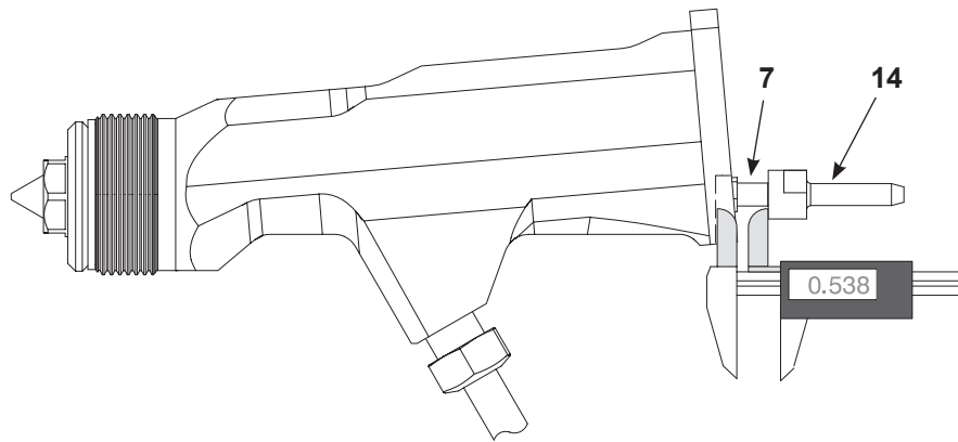
Figure 7-7 Packing Cartridge Replacement – Removing Trigger Puller
