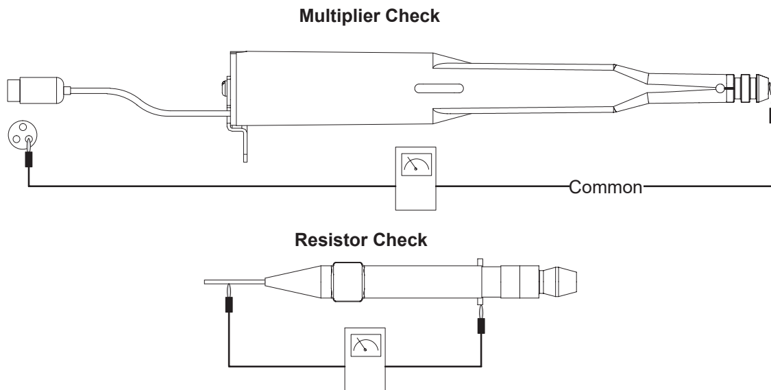
Figure 6-2 Multiplier and Needle Continuity and Resistance Check
