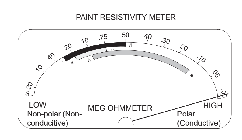
Figure 3-2 Resistivity Range for Coatings
