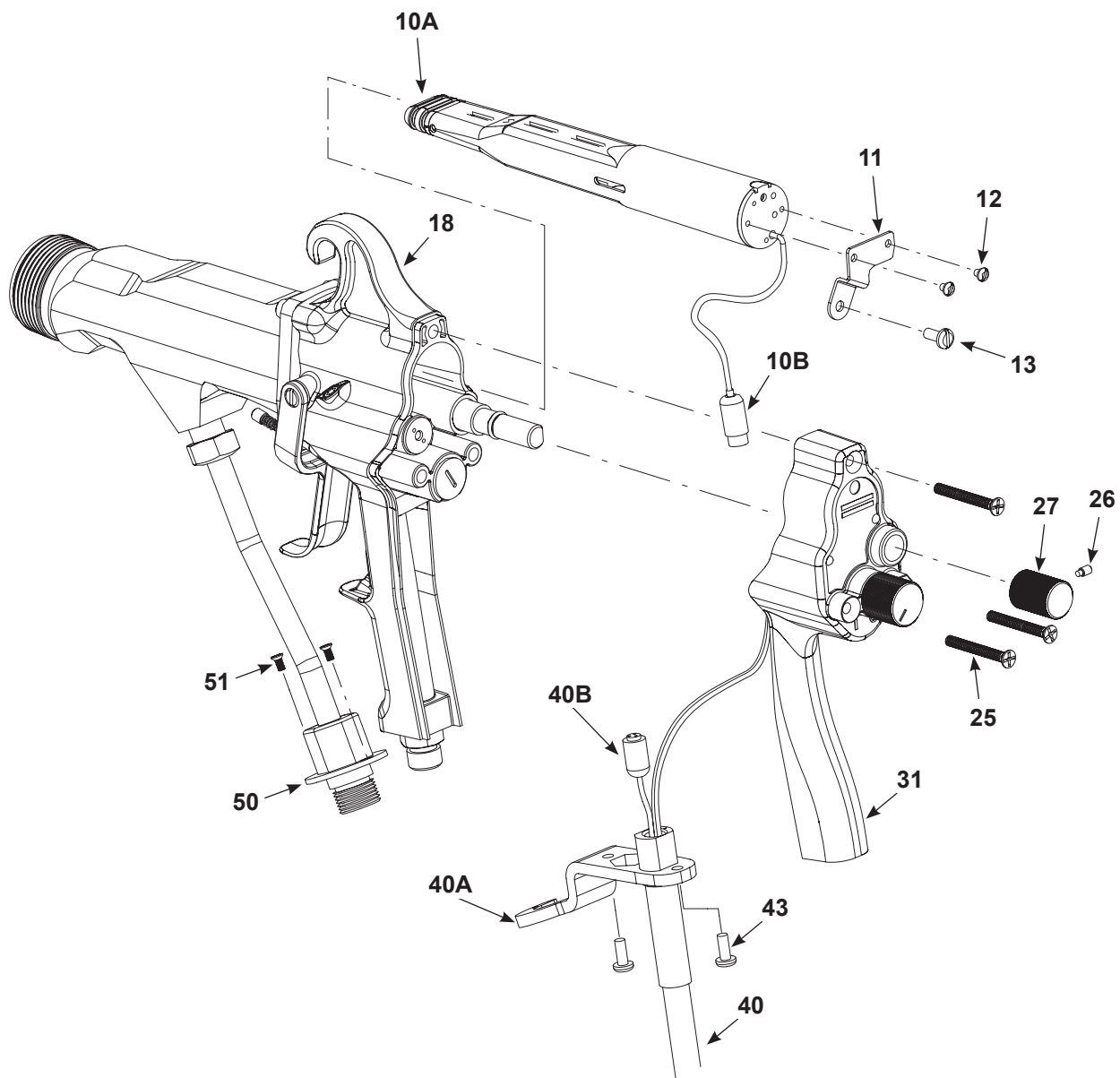
Figure 7-10 Multiplier Replacement
