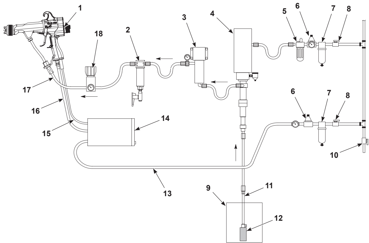
1. Spray gun 7. Air filter 13. Air supply hose 2. Fluid filter 8. Self-relieving shutoff valve 14. Control unit 3. Fluid heater 9. Fluid supply 15. Gun cable 4. Pump 10. Drain valve 16. Air hose 5. Air lubricator 11. Siphon rod 17. Fluid hose 6. Air regulator 12. Siphon screen 18. Fluid pressure regulator
