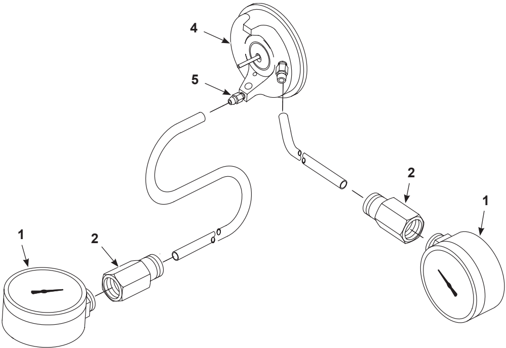
Figure 8-2 HVLP Compliance Kit
