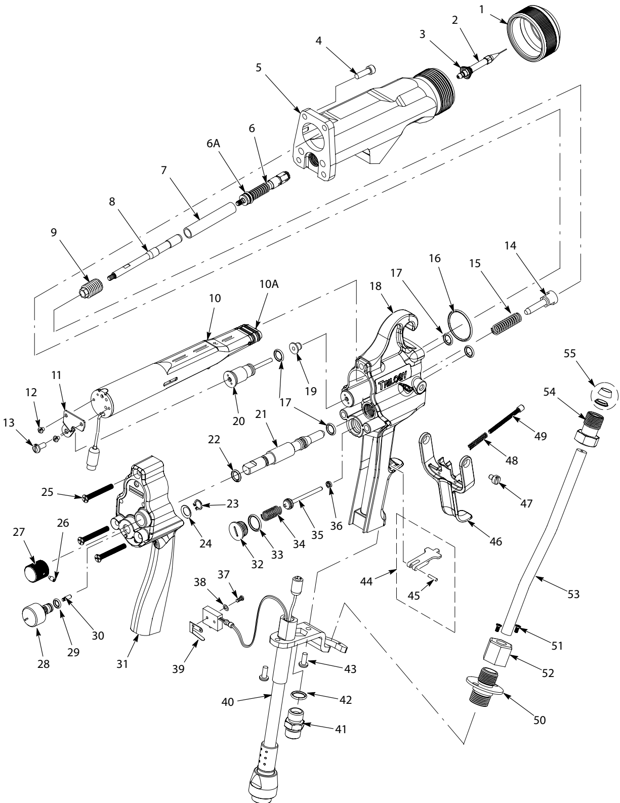
Figure 8-1 Spray Gun Parts
