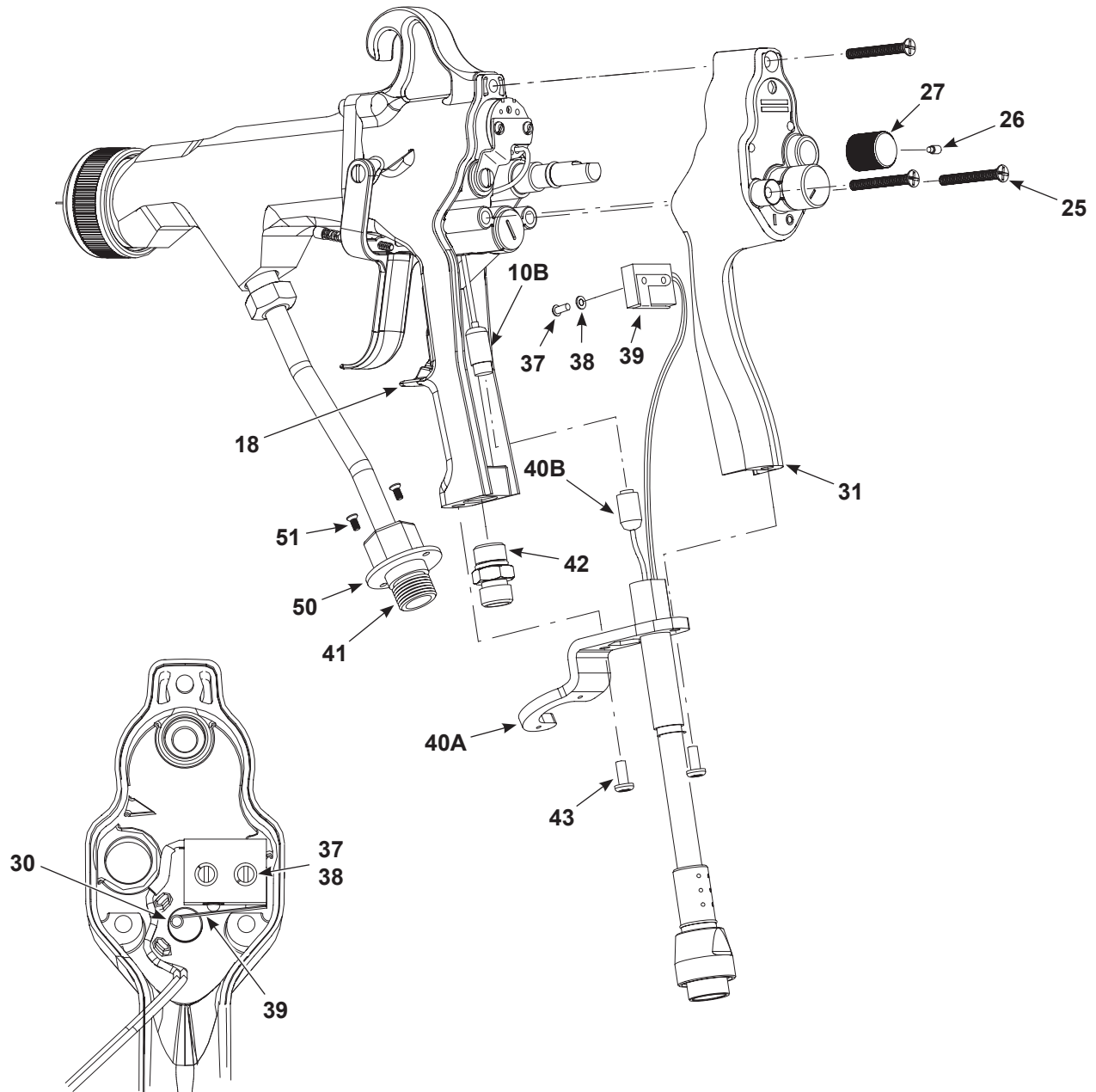
Figure 7-8 Cable Air Inlet Fitting Replacement
