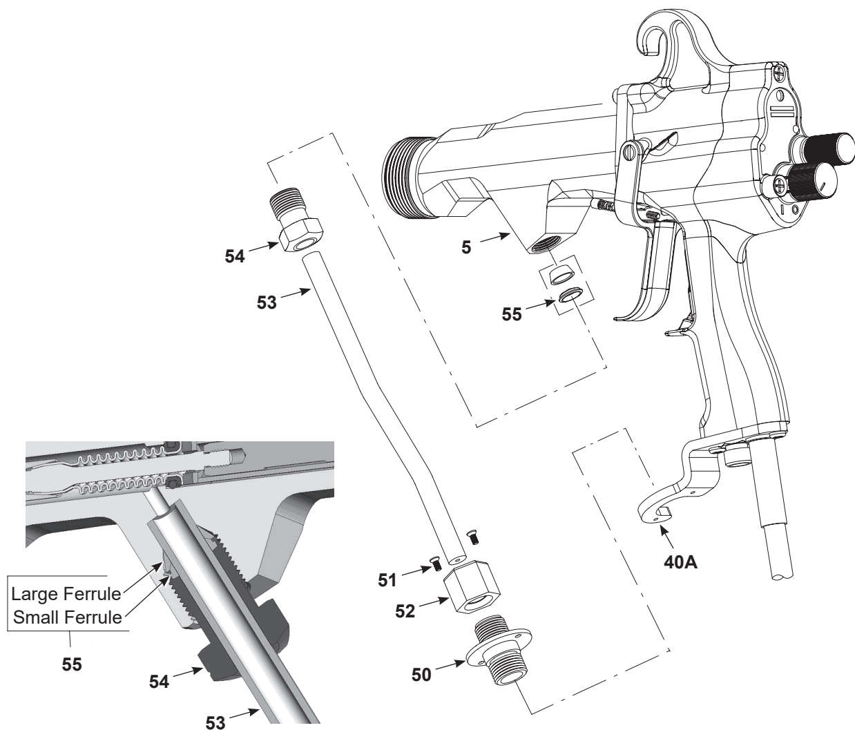
Figure 7-11 Multiplier Replacement
