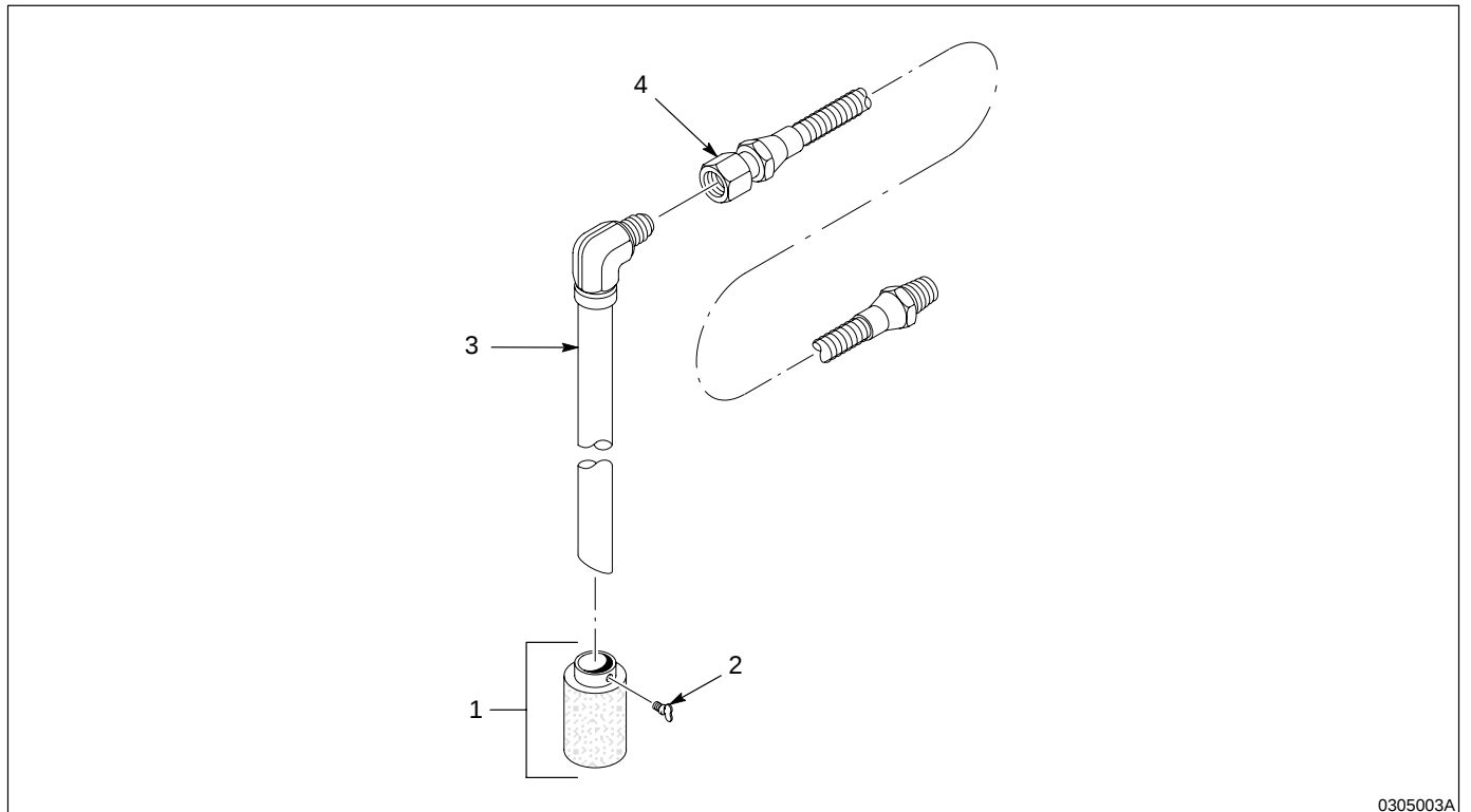
Fig. 2 Stainless Steel 1-Inch Siphon Accessory Group
