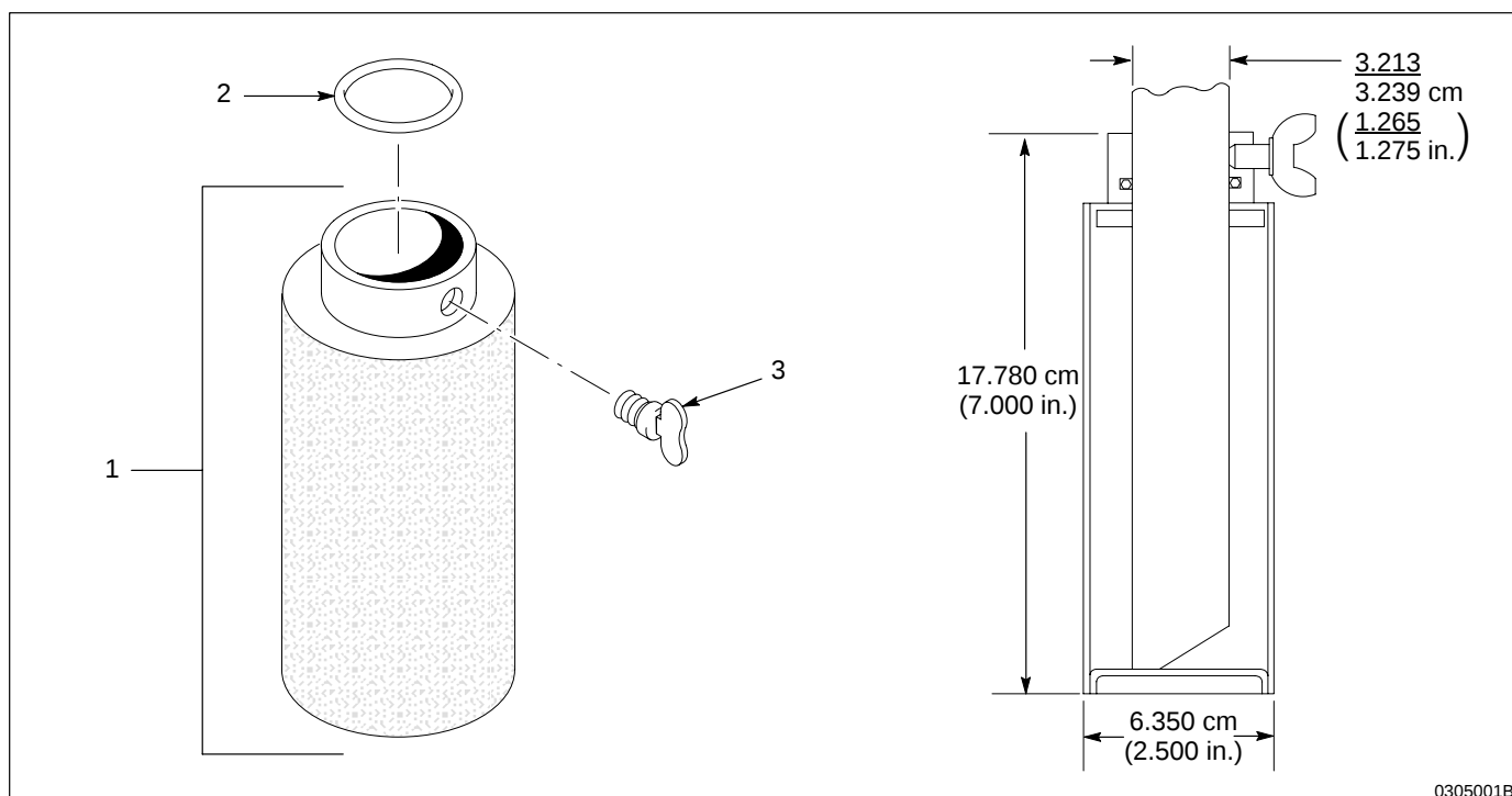
Fig. 1 Siphon Strainer Assemblies for 180C, 25B, 180D/360D, and 32/64 Pumps
