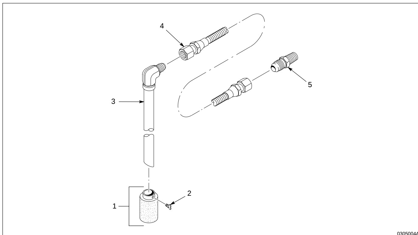
Fig. 3 Stainless Steel 1-Inch Siphon Accessory Group
