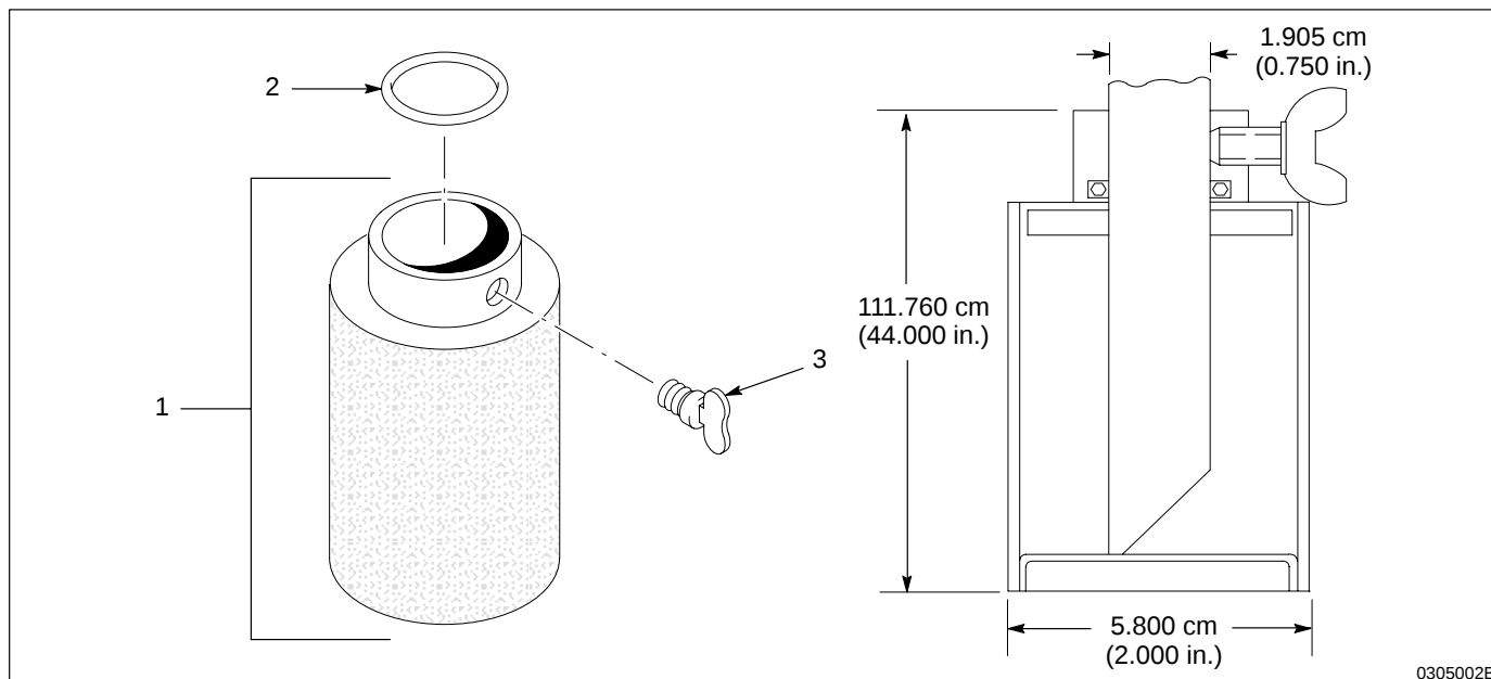
Fig. 4 Siphon Strainer Assemblies for 25B and 64B Pumps
