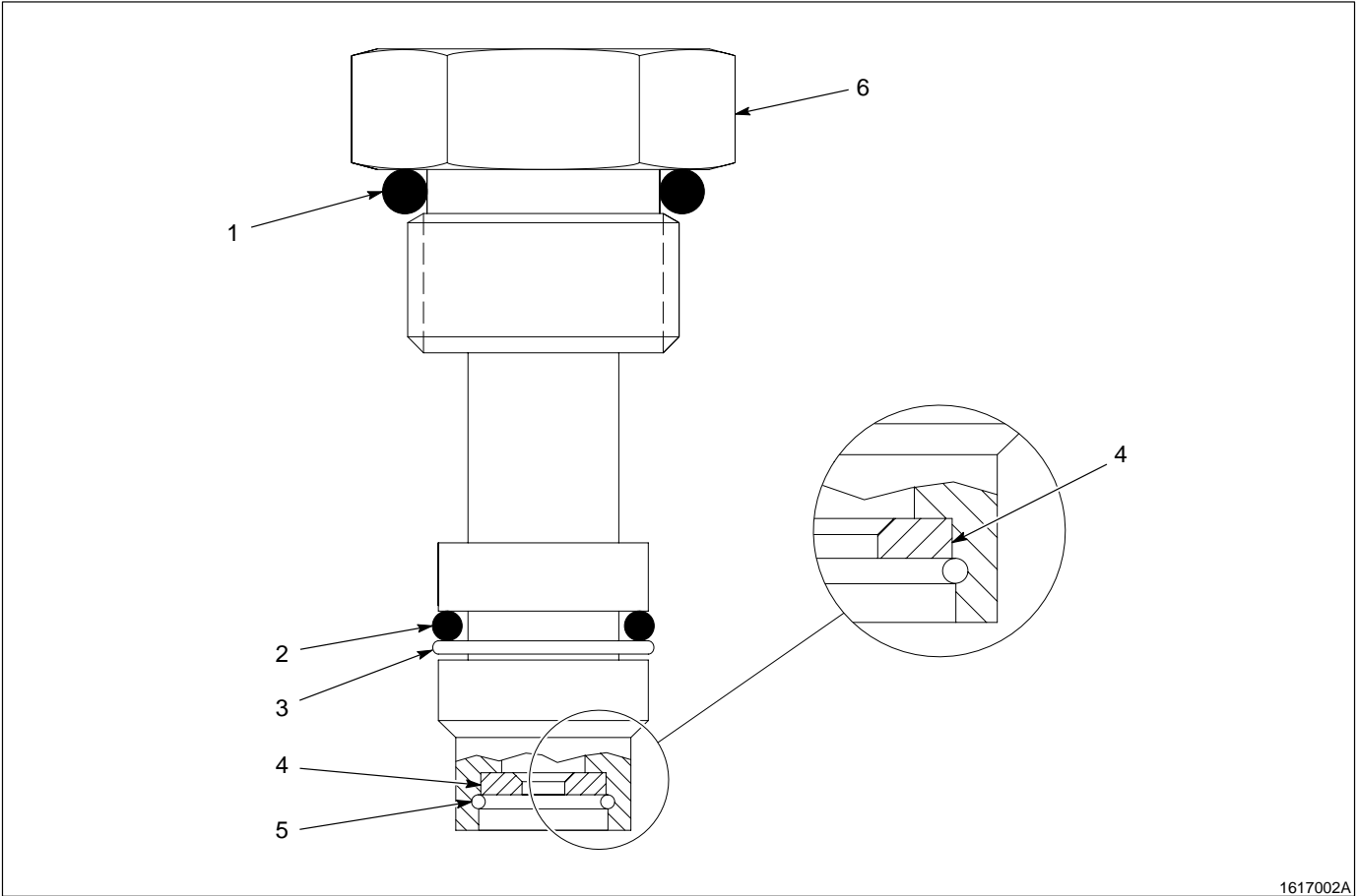
Fig. 2 Orifice Kits Note: Install the chamfered restrictor (4) as shown in Figure 2.
