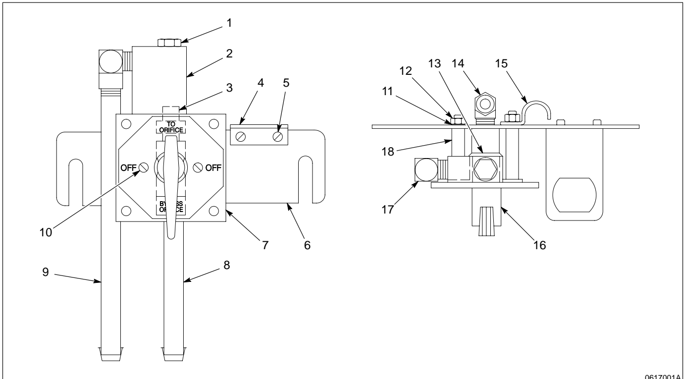
Fig. 1 Fixed Orifice Circulation Valve
