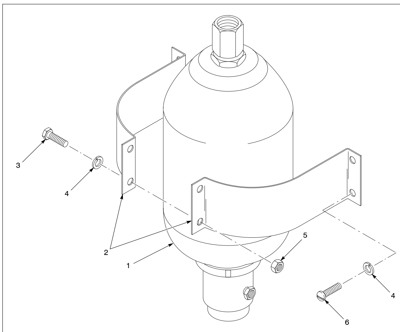
Figure 3 Accumulator and Bracket Parts
