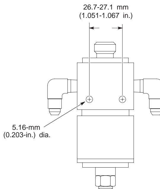
Figure 2 A10A Mounting Dimensions
