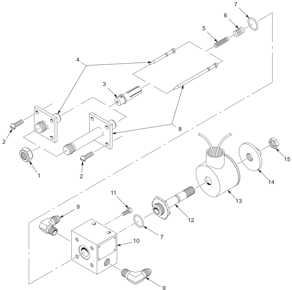
Figure 5 Exploded View of Model A10A Automatic Electric Spray Gun (Standard Needle and Seat and 2.5-in. Extension Shown)
