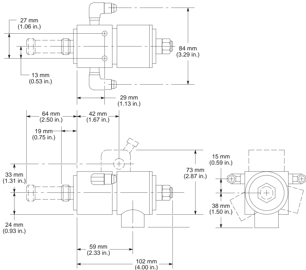
Figure 6 Model A10A Automatic Electric Spray Gun Dimensions
