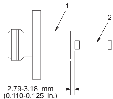
Figure 4 Needle Position When Properly Seated
