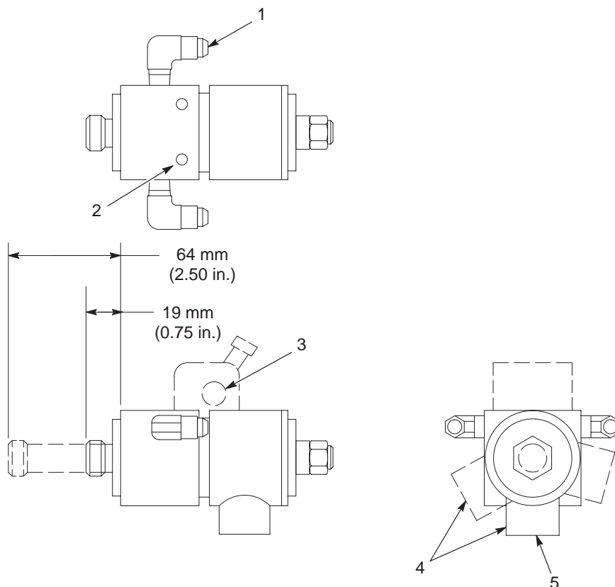
Figure 3 Key Mounting and Connection Points of the A10A Gun
