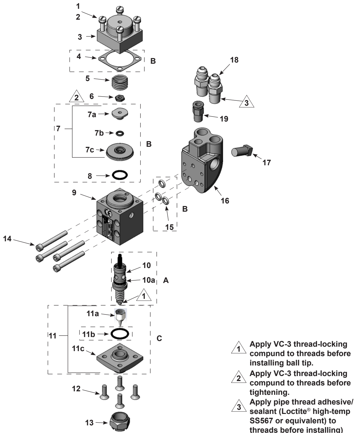
Figure 7 Single Gun with Needle and Seat Parts
