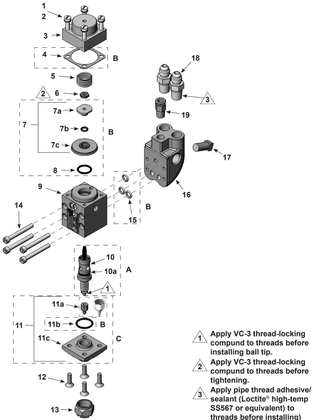
Figure 6 Single Gun with Ball and Seat Parts
