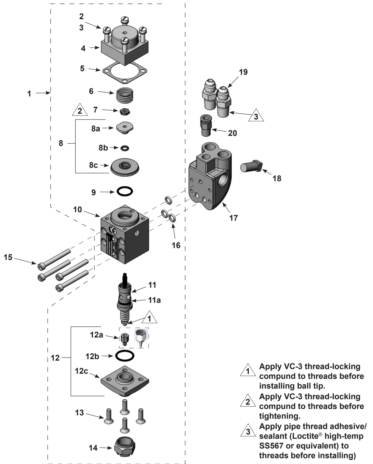
Figure 4 Single Gun Repair
