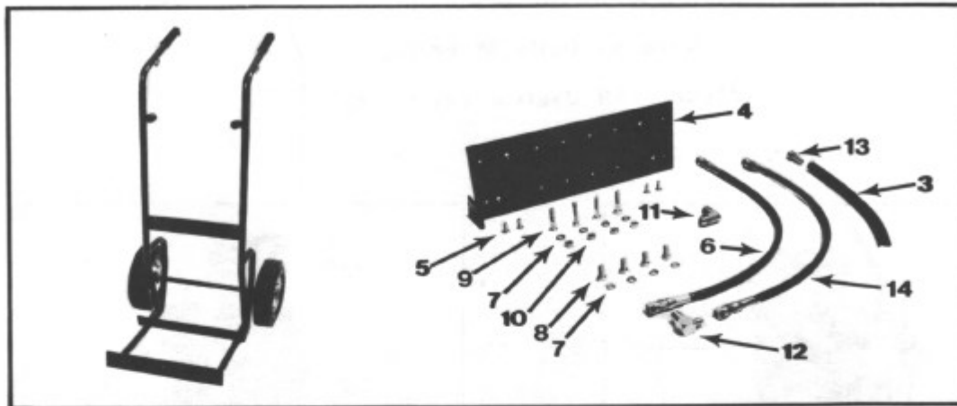
Figure 11 - Dolly with Mount
