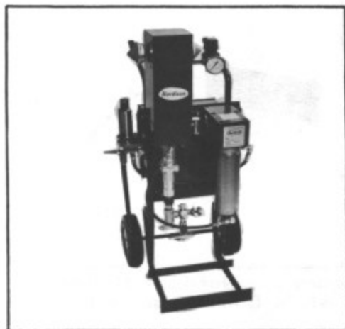
Figure 3 - Model 25B, NH-4 Heater, Filter, and EPU-8 Power Unit, Front View
