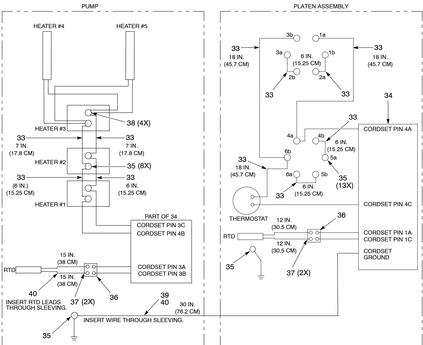
Figure 3 Platen Assembly Parts (continued)
