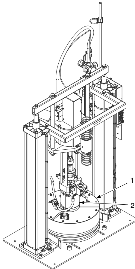
Figure 1 Low Wattage Heated Platen and Cable Assembly ( Cable assembly not shown. )
