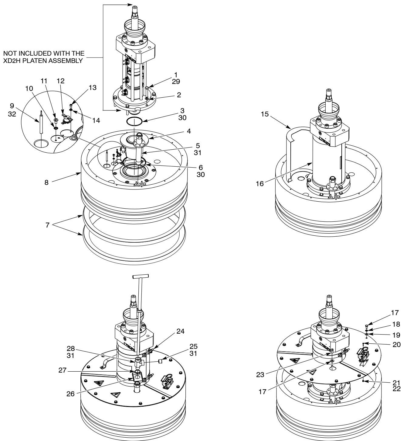
Figure 2 XD2H platen assembly parts
