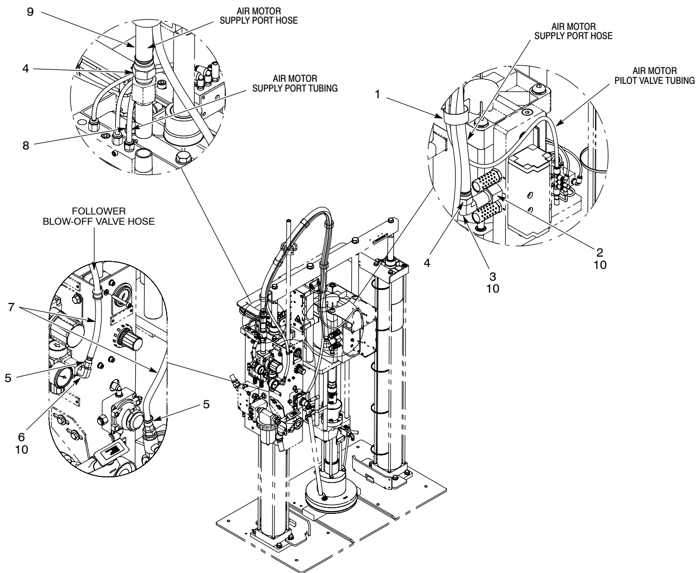
Figure 2 5/30-Gallon Large Frame Hybrid Hose Module
