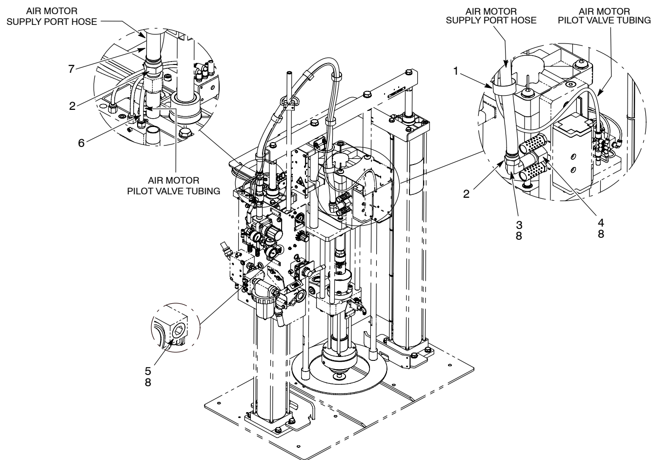
Figure 4 Large Frame Mini-Tote Fire Resistant Hose Module
