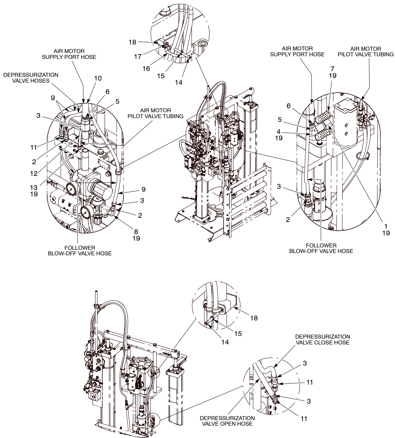
Figure 5 55-Gallon Black Hose Modules
