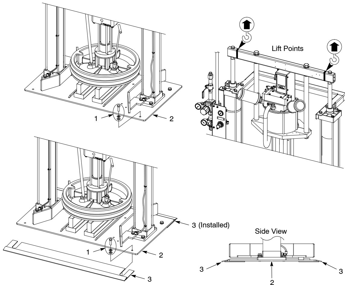
Figure 3 Installing the Adapter Plates
