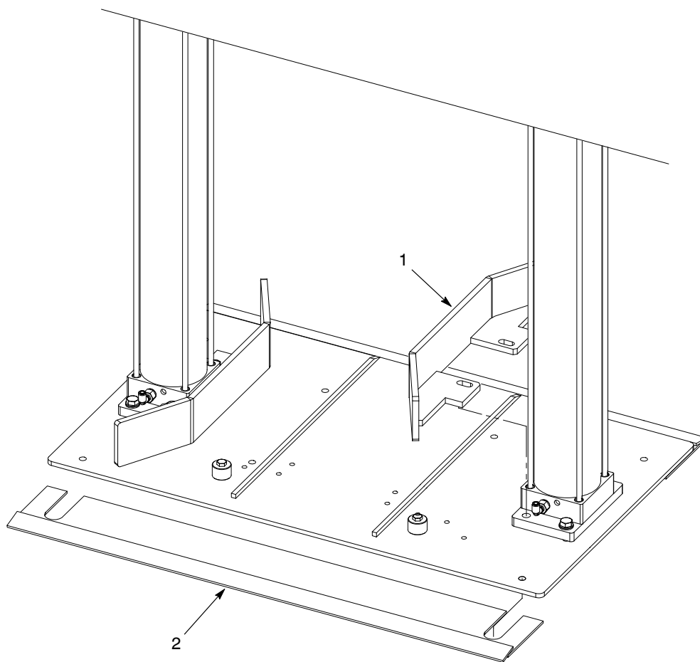
Figure 4 Drum Cart Frame Adapter Plate Parts
