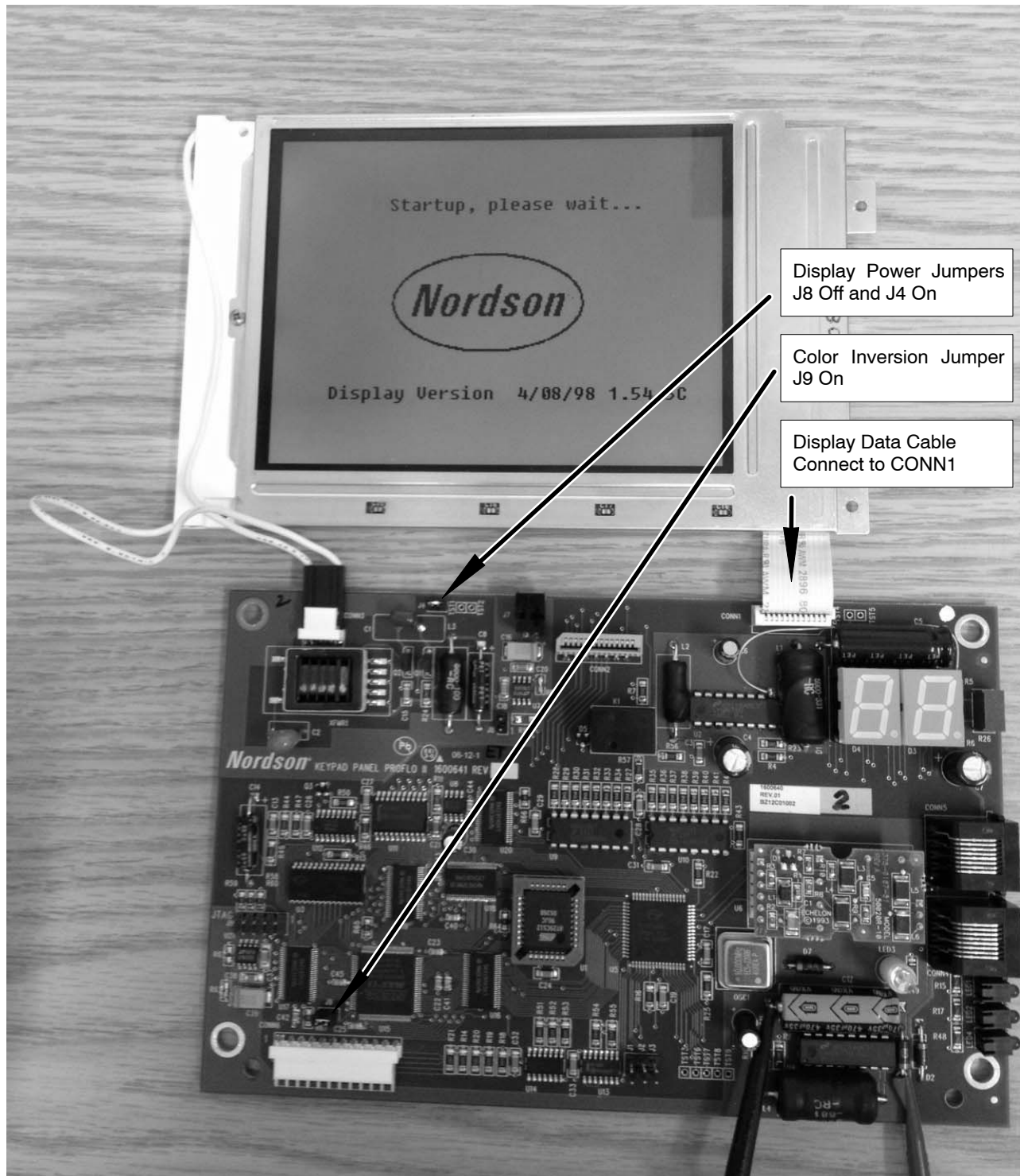
Figure 2 Old Display with New Keypad PCA (New PCA Only 1604380)
