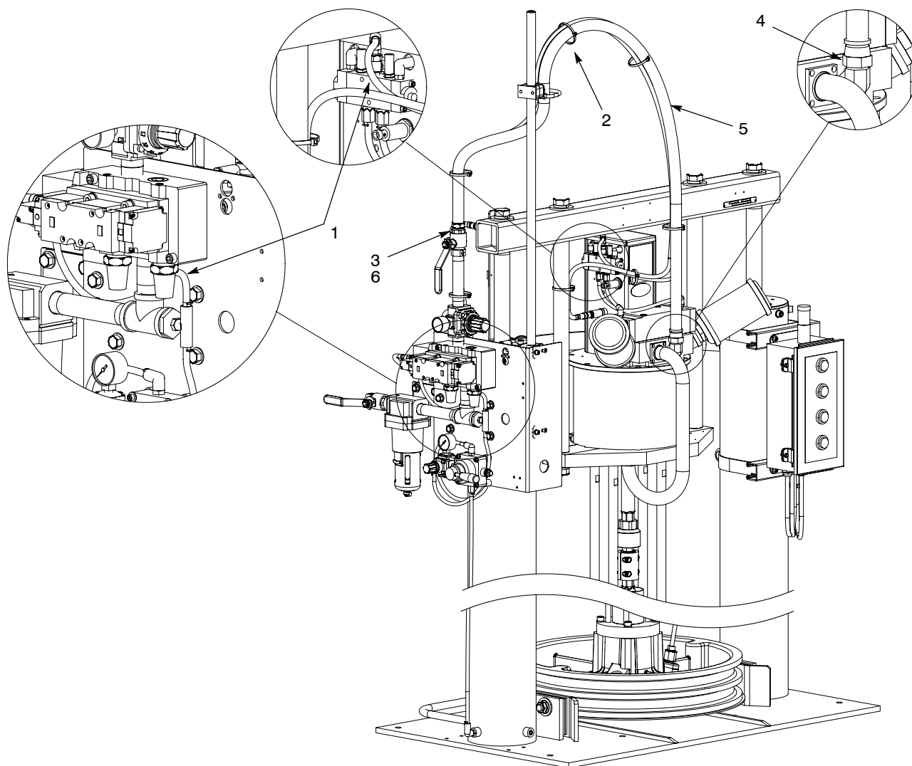
Figure 2 Parts
