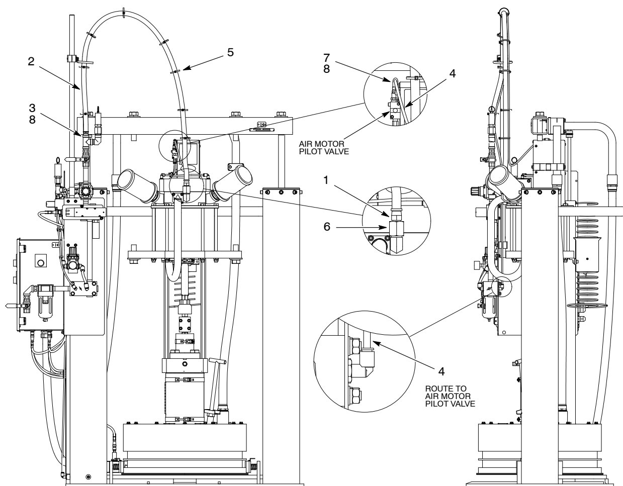
Figure 2 XD2H Standard Hose Module Parts
