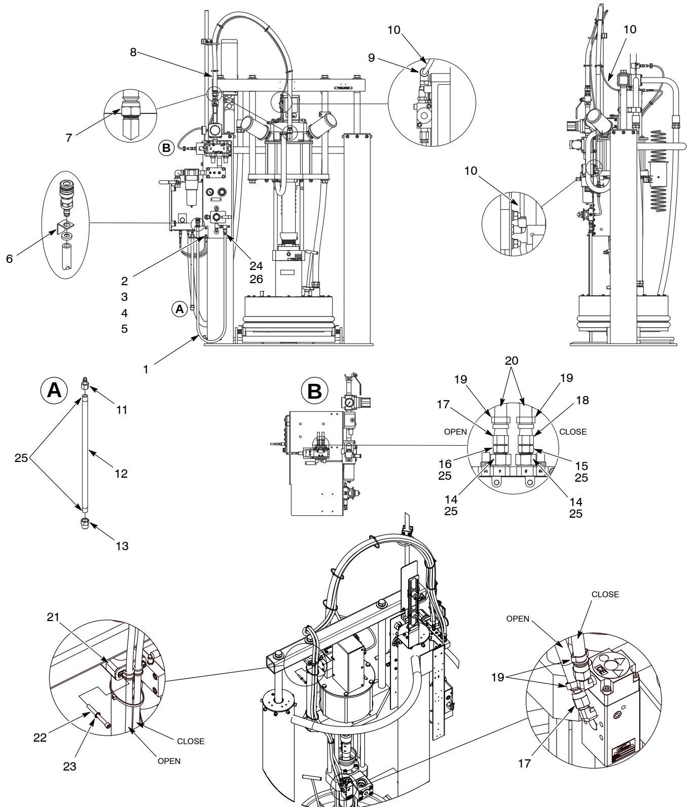
Figure 3 XD2H Hose Module with Depressurization Parts
