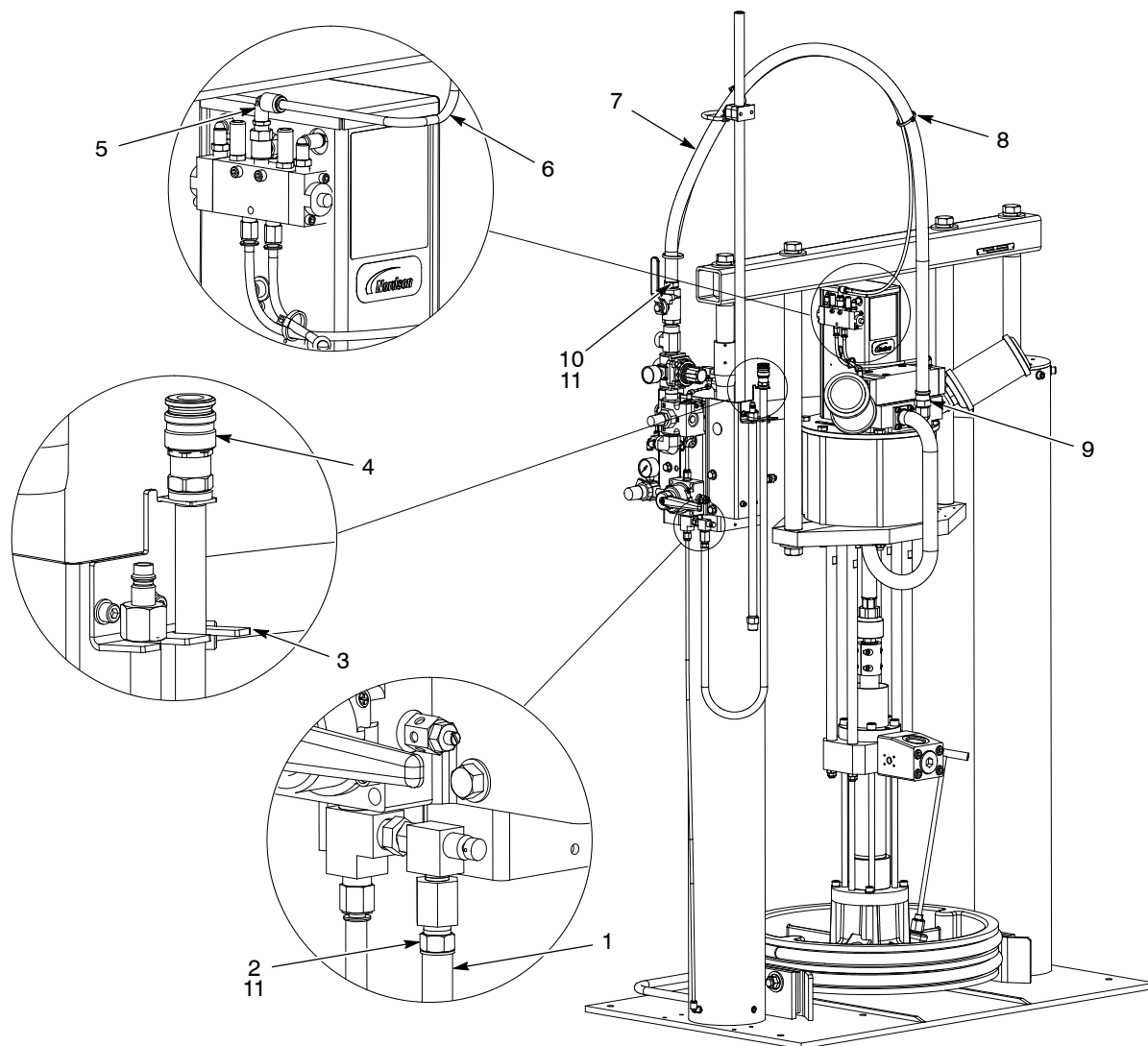
Figure 19 Rhino VE Large Frame CE Hose
