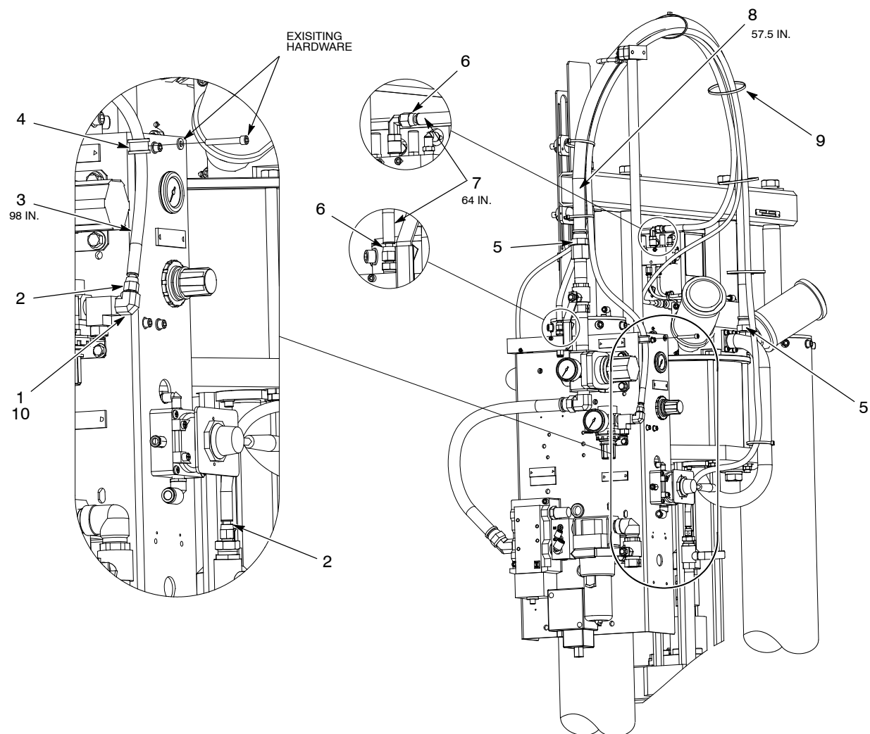
Figure 10 55-Gallon Large Frame Fire Resistant Hose
