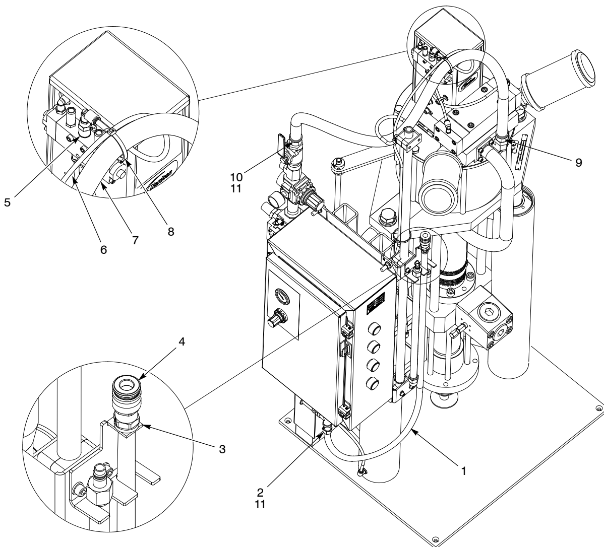
Figure 18 Rhino VE Small Frame CE Hose
