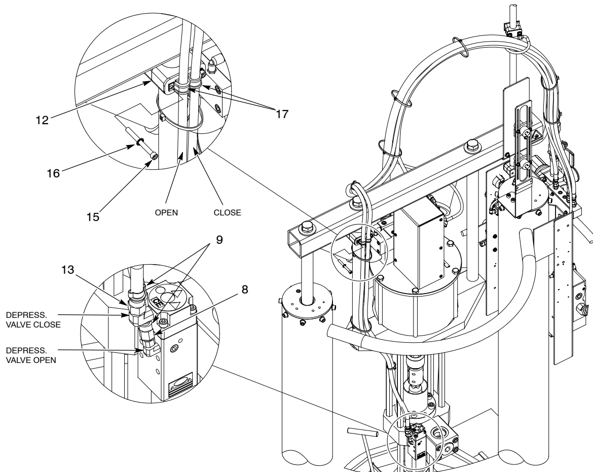
Figure 16 55-Gallon Large Frame Black Hose with Depressurization (continued)
