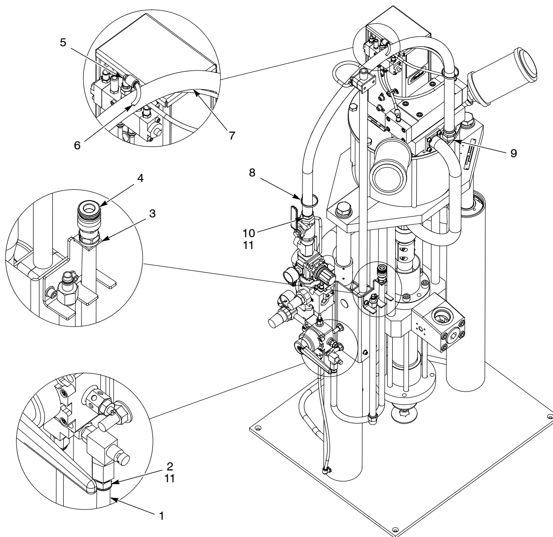
Figure 17 Rhino VE Small Frame Hose
