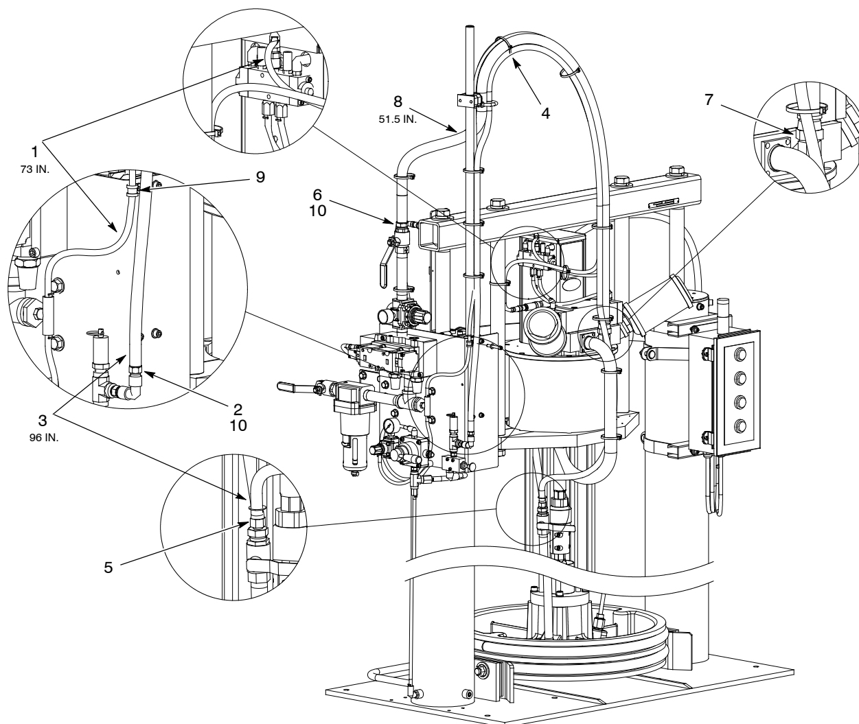
Figure 11 55-Gallon Large Frame Green Fire Resistant Hose
