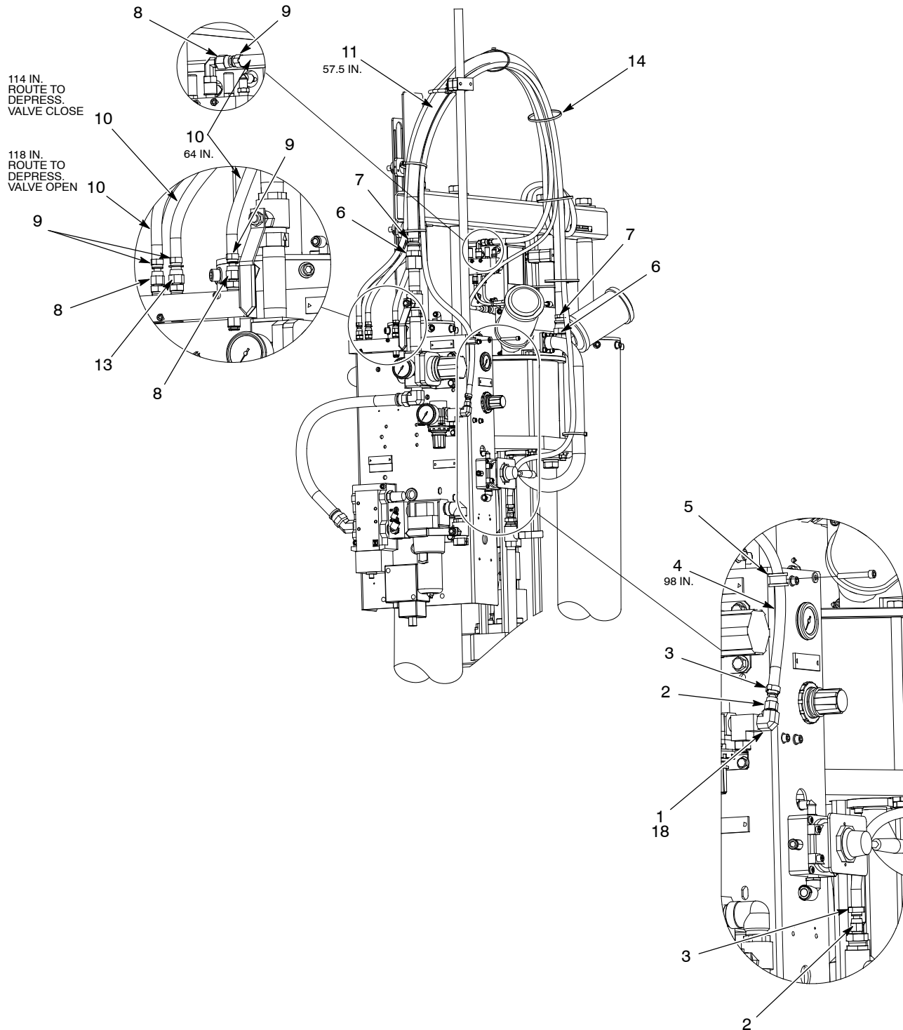
Figure 15 55-Gallon Large Frame Black Hose with Depressurization
