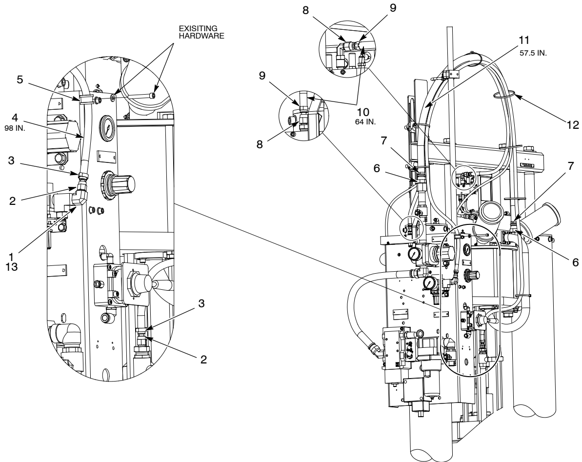
Figure 12 55-Gallon Large Frame Black Hose
