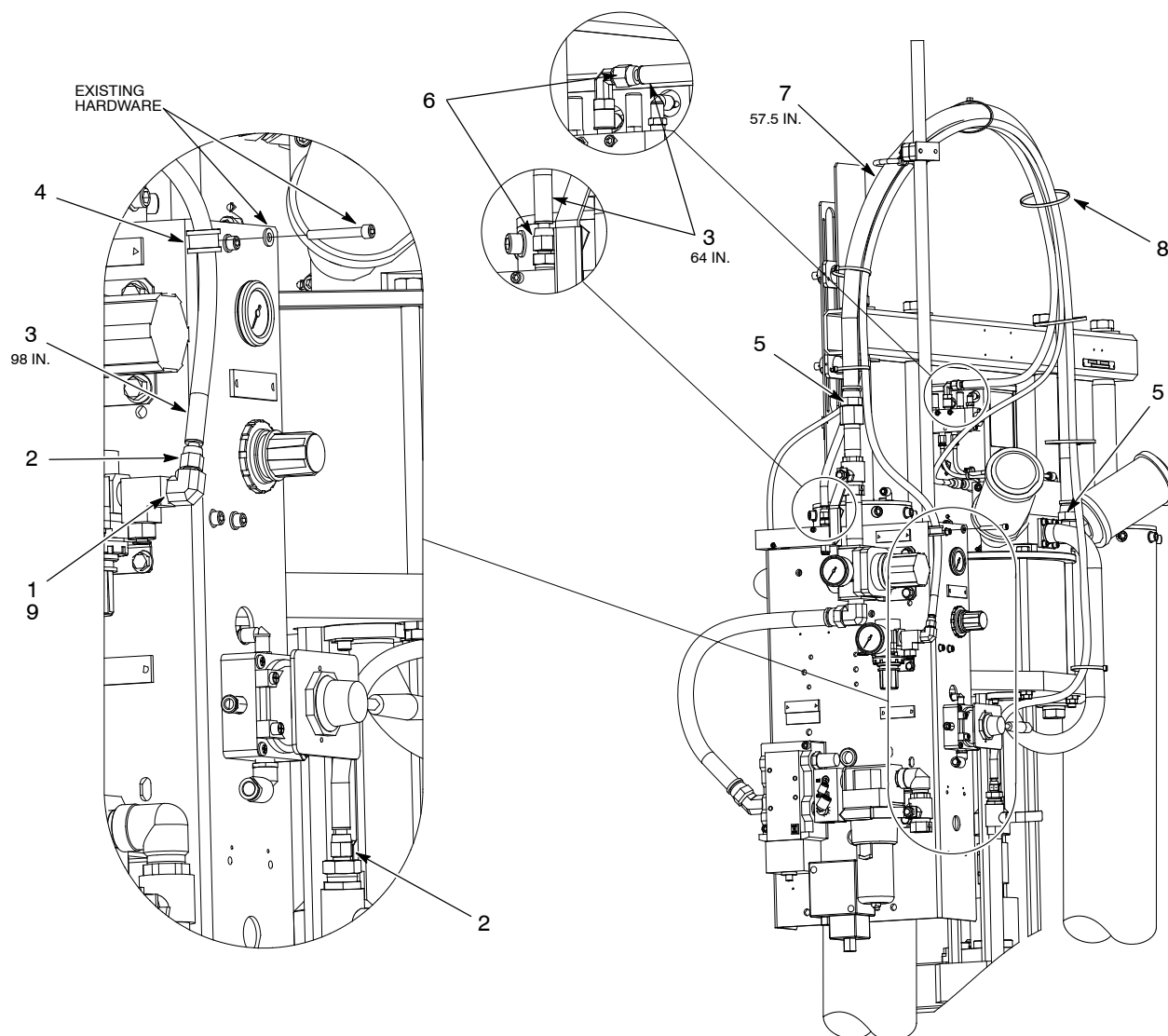
Figure 4 5/30-Gallon Large Frame Fire Resistant Hose
