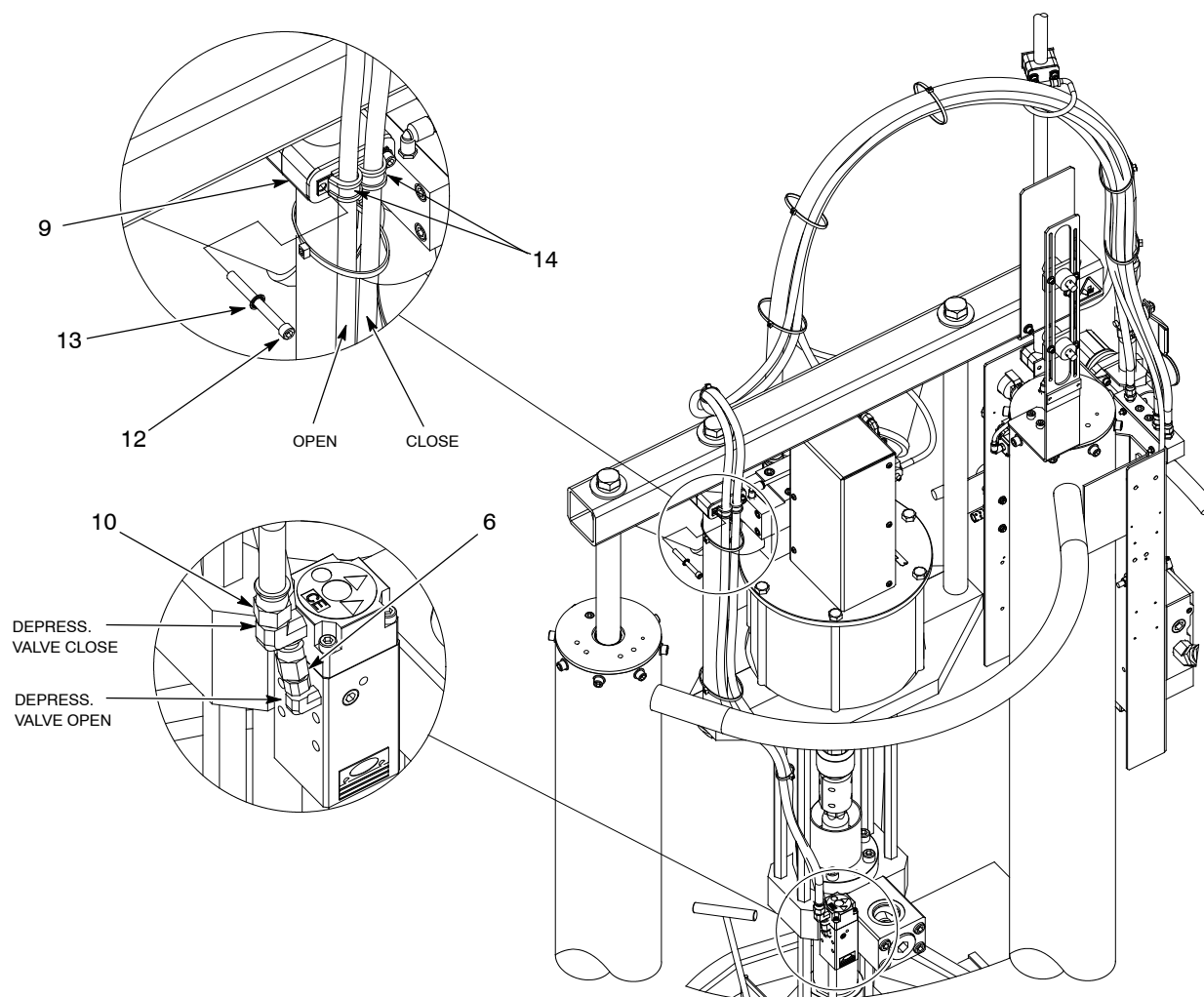
Figure 14 55-Gallon Large Frame Black Hose ( continued )
