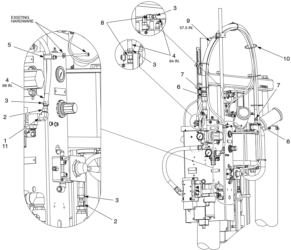
Figure 5 5/30-Gallon Large Frame Black Hose
