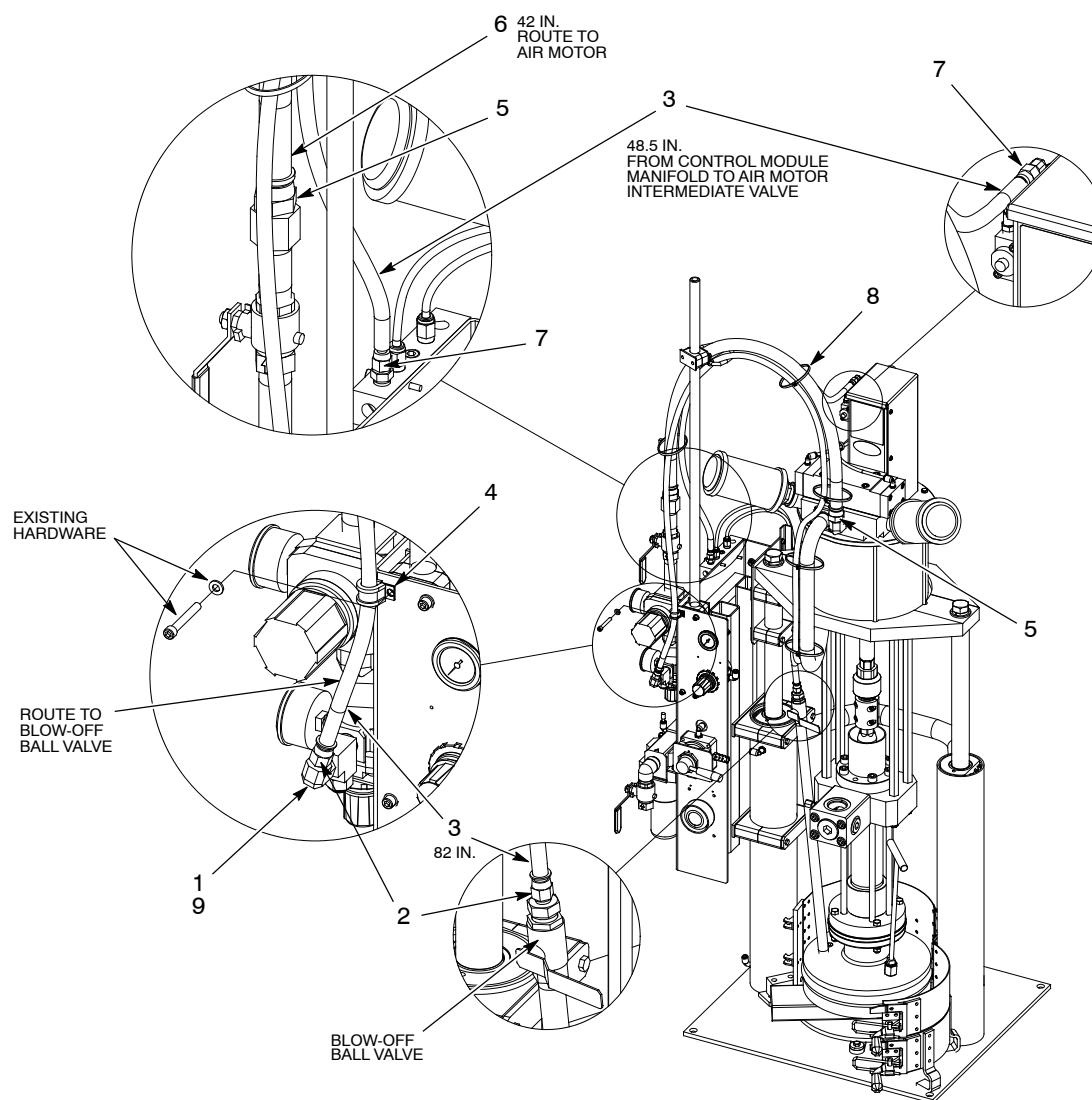
Figure 2 Small Frame Fire Resistant Interconnect Hose Module
