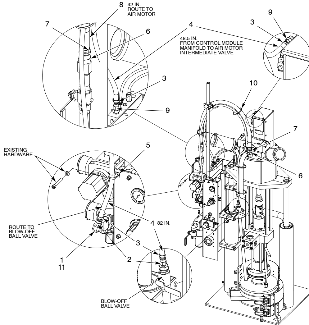
Figure 3 Small Frame Black Hose
