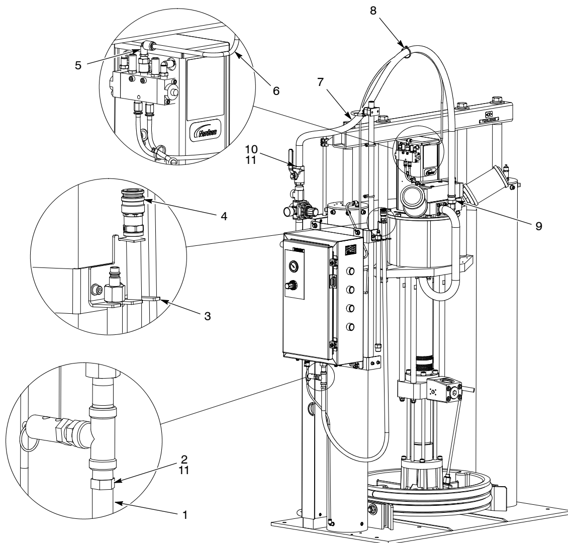
Figure 20 Rhino VE Large Frame CE Hose
