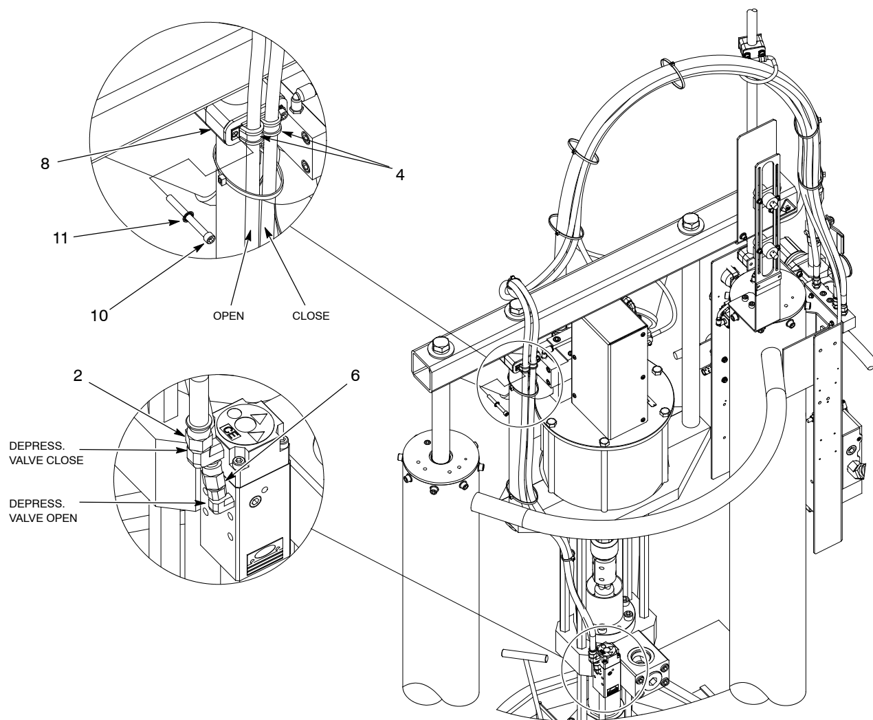
Figure 7 5/30-Gallon Large Frame Fire Resistant Hose with Depressurization ( continued )
