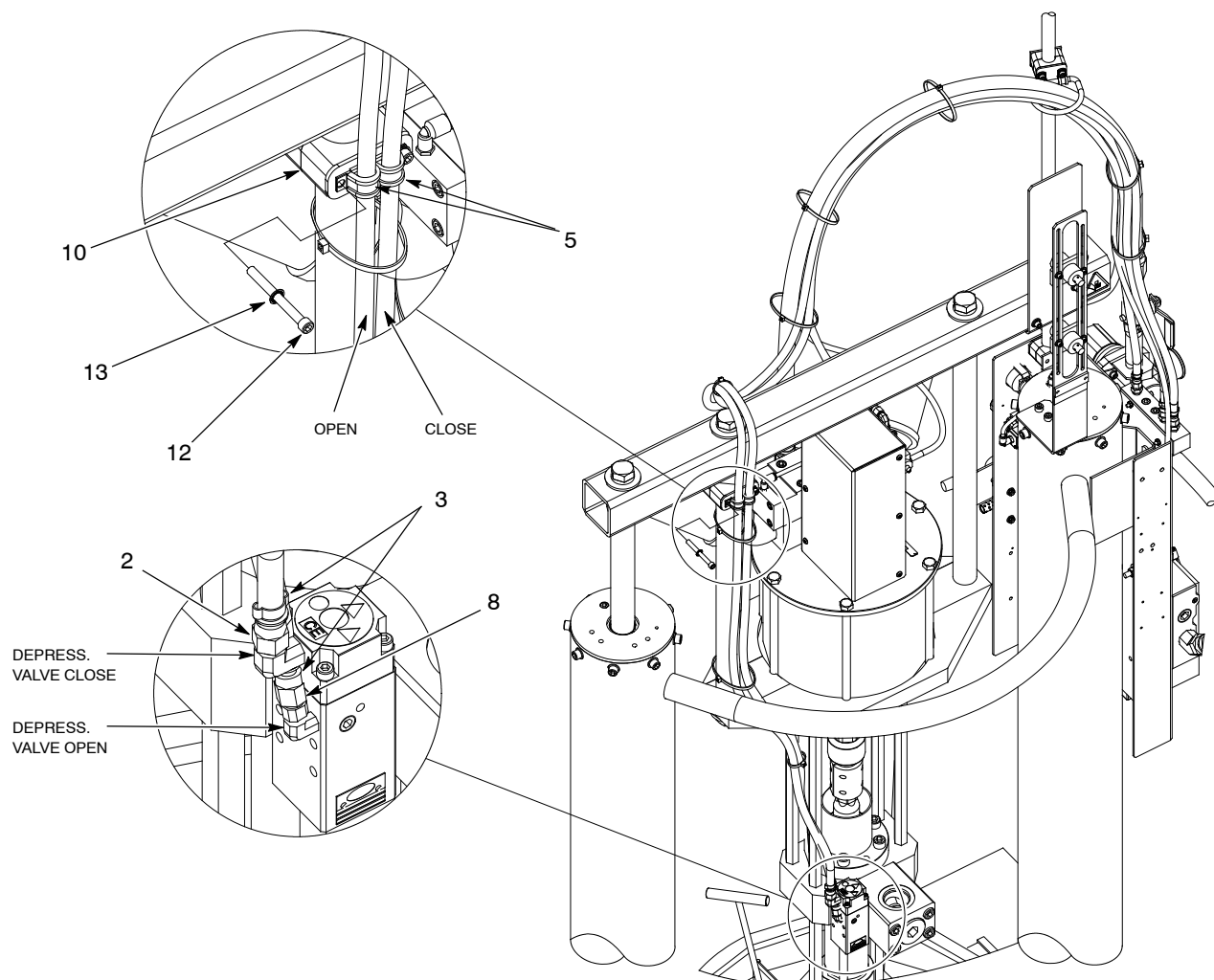
Figure 9 5/30-Gallon Large Frame Black Hose with Depressurization ( continued )
