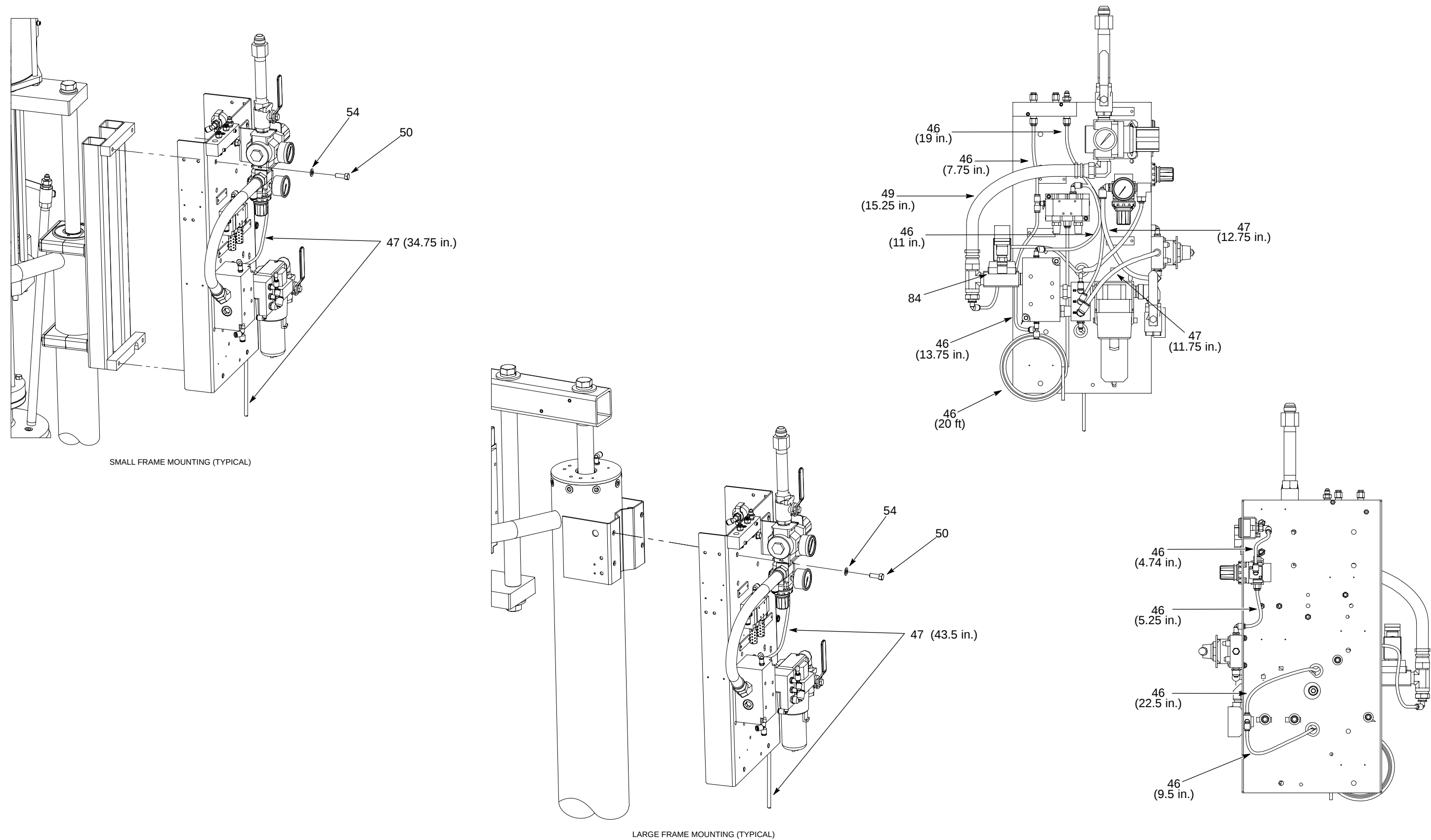
Figure 9 Control Module Parts
