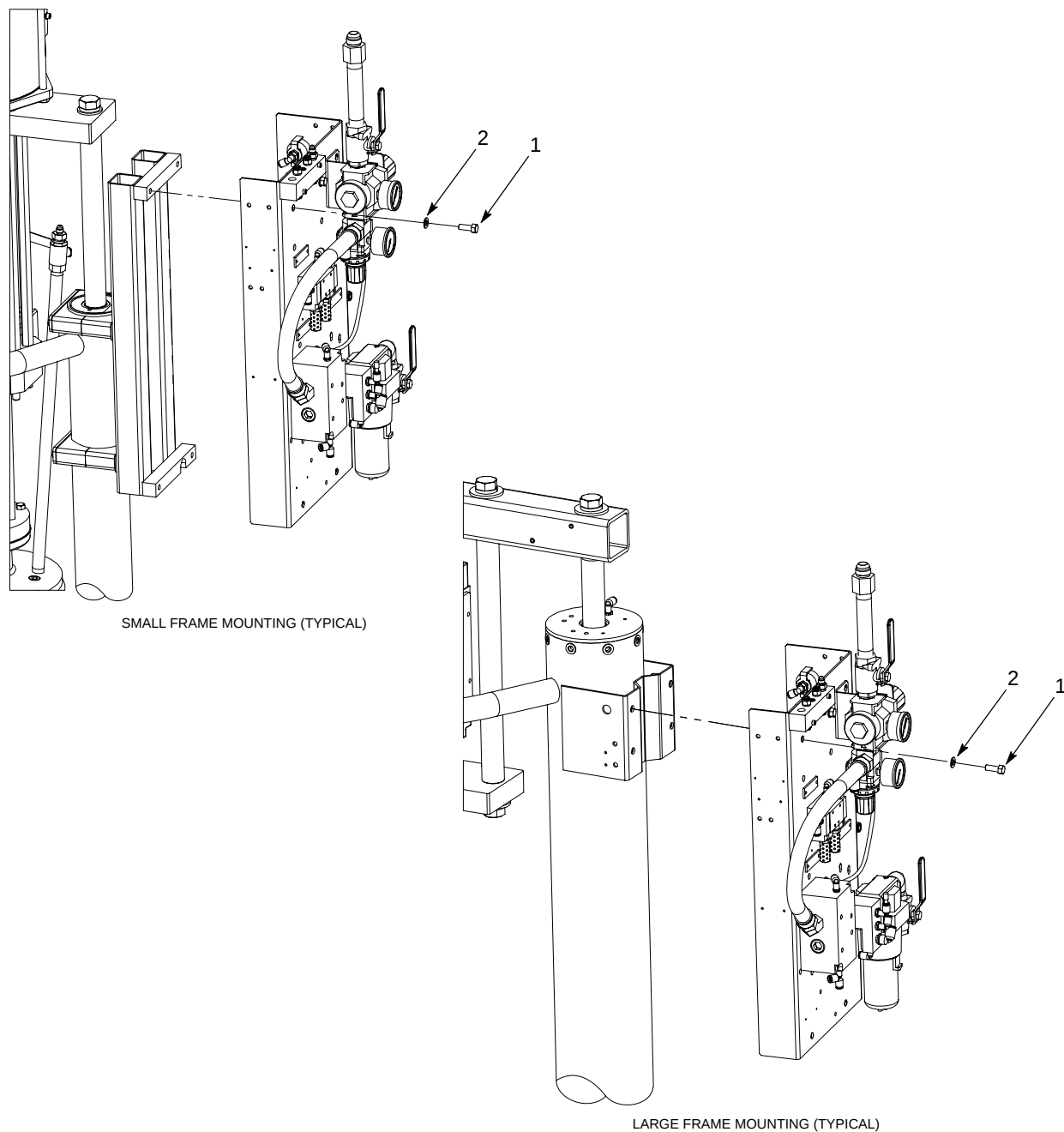
Figure 3 Installing a Control Module
