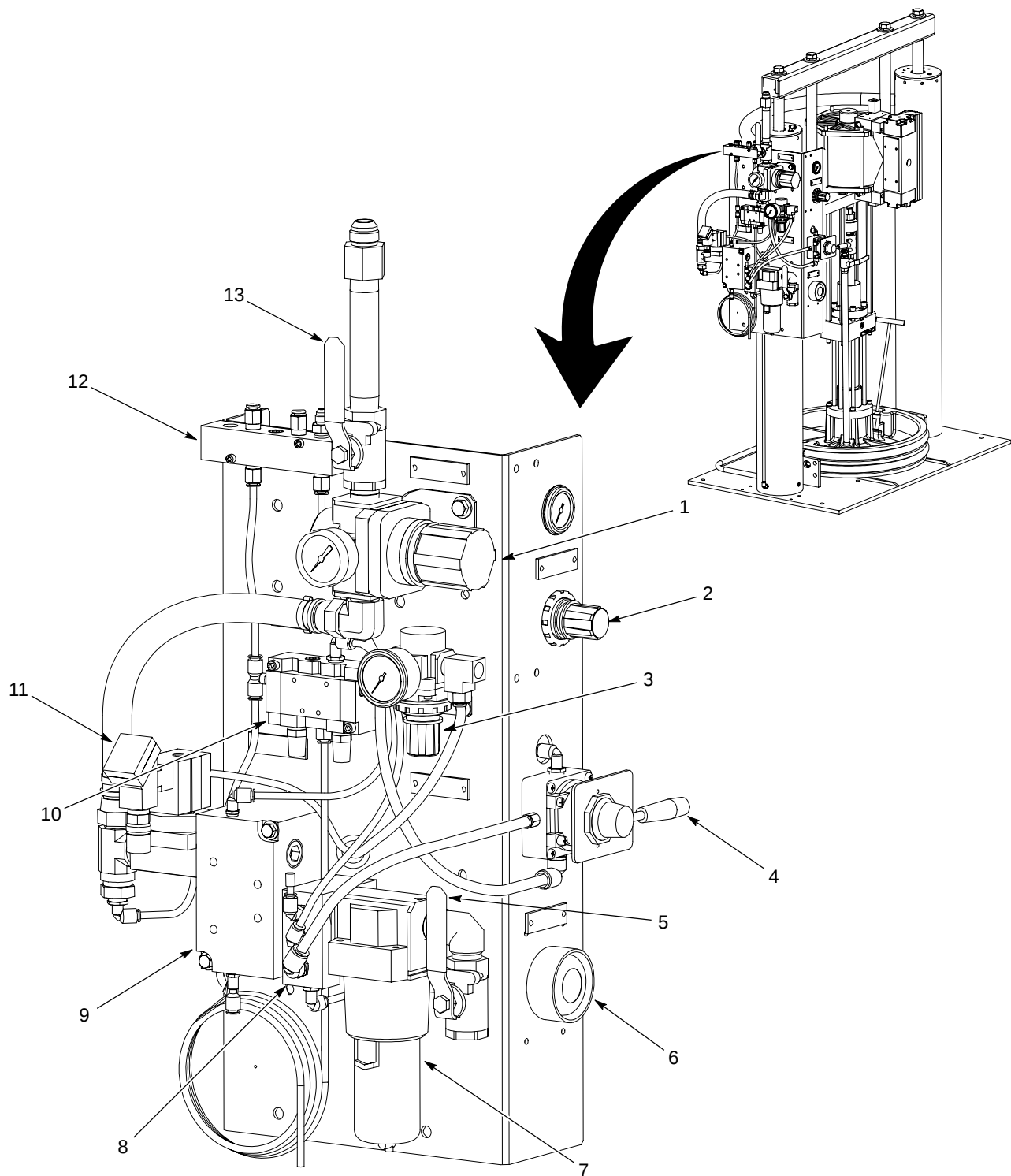
Figure 2 Control Module Components
