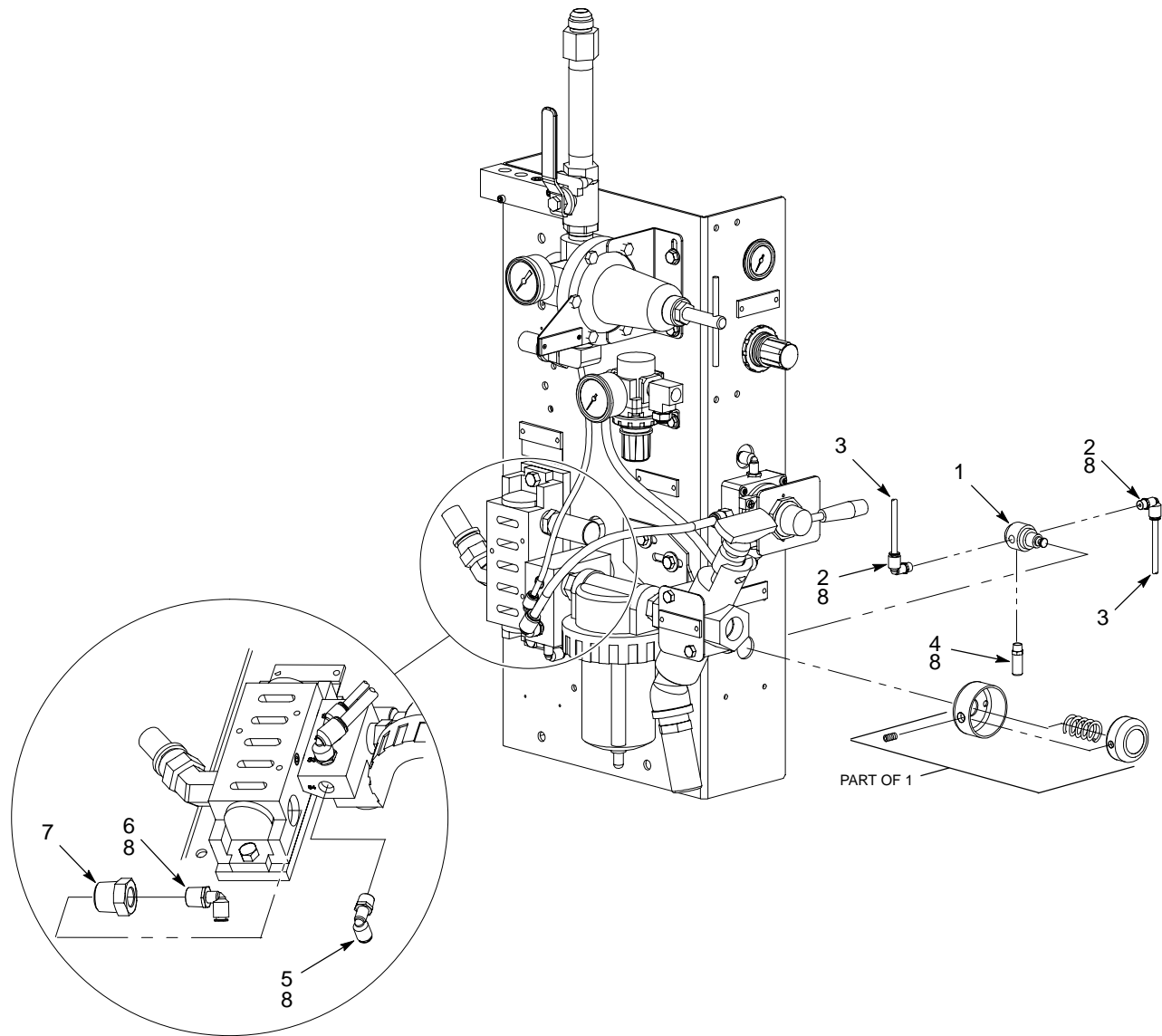
Figure 2 Parts
