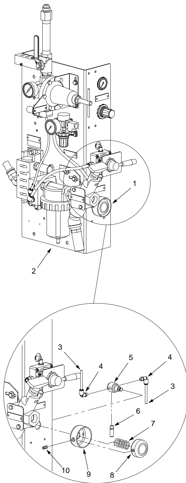
Figure 1 Rhino SD/XD Type-F Electric Control Module Pneumatic Purge Button
