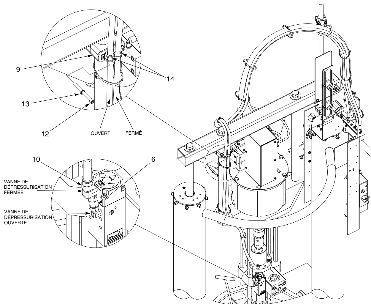
Figure 14 Tuyau noir grand châssis 55 gallons (210 l) (suite)
