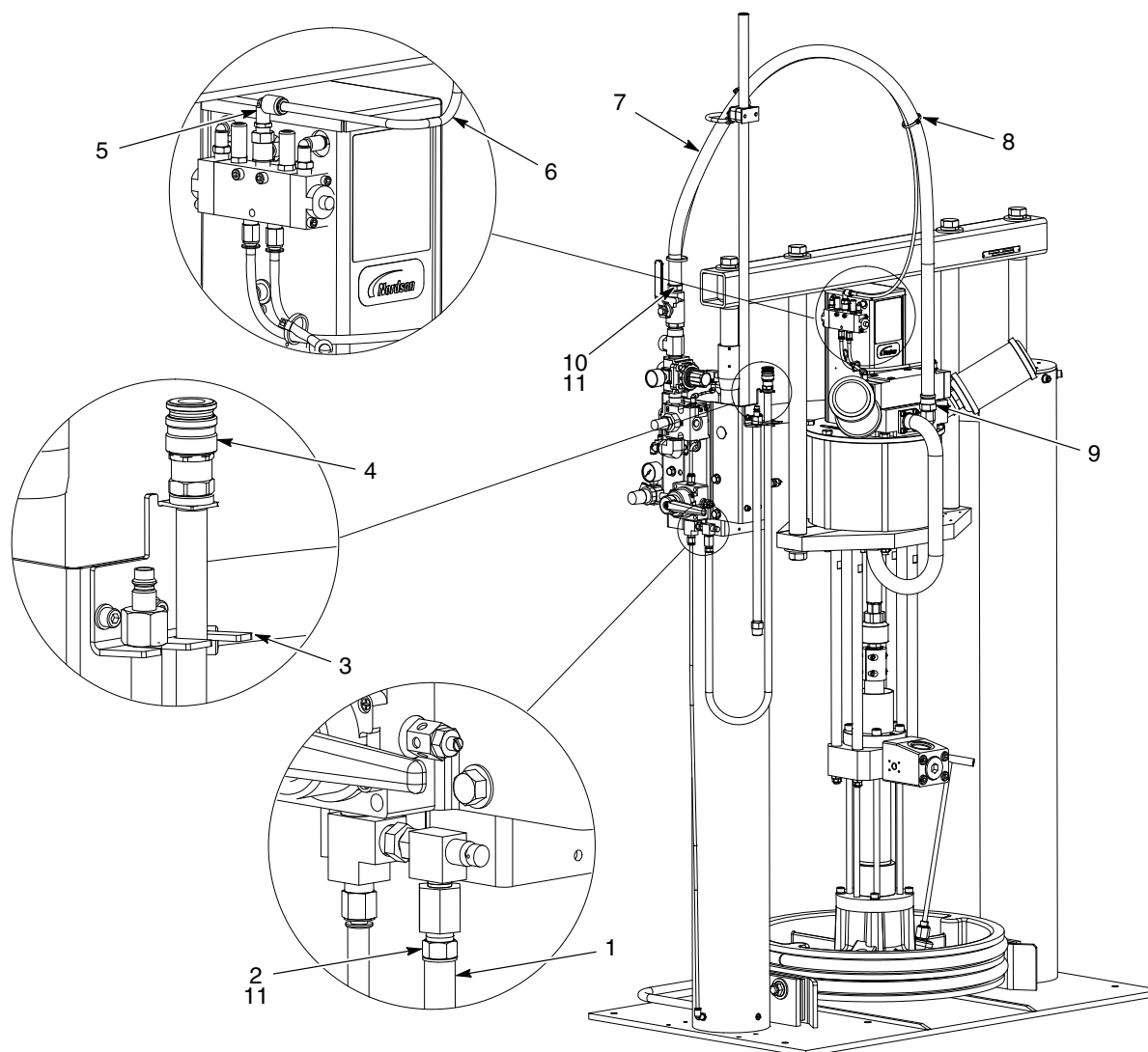
Figure 19 Tuyau CE grand châssis Rhino VE
