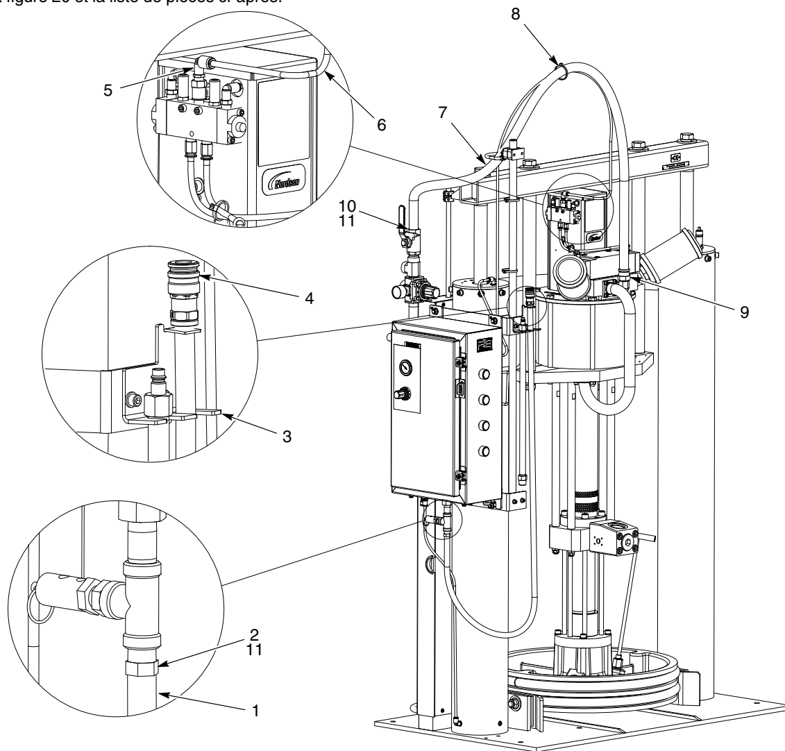
Figure 20 Tuyau CE grand châssis Rhino VE
