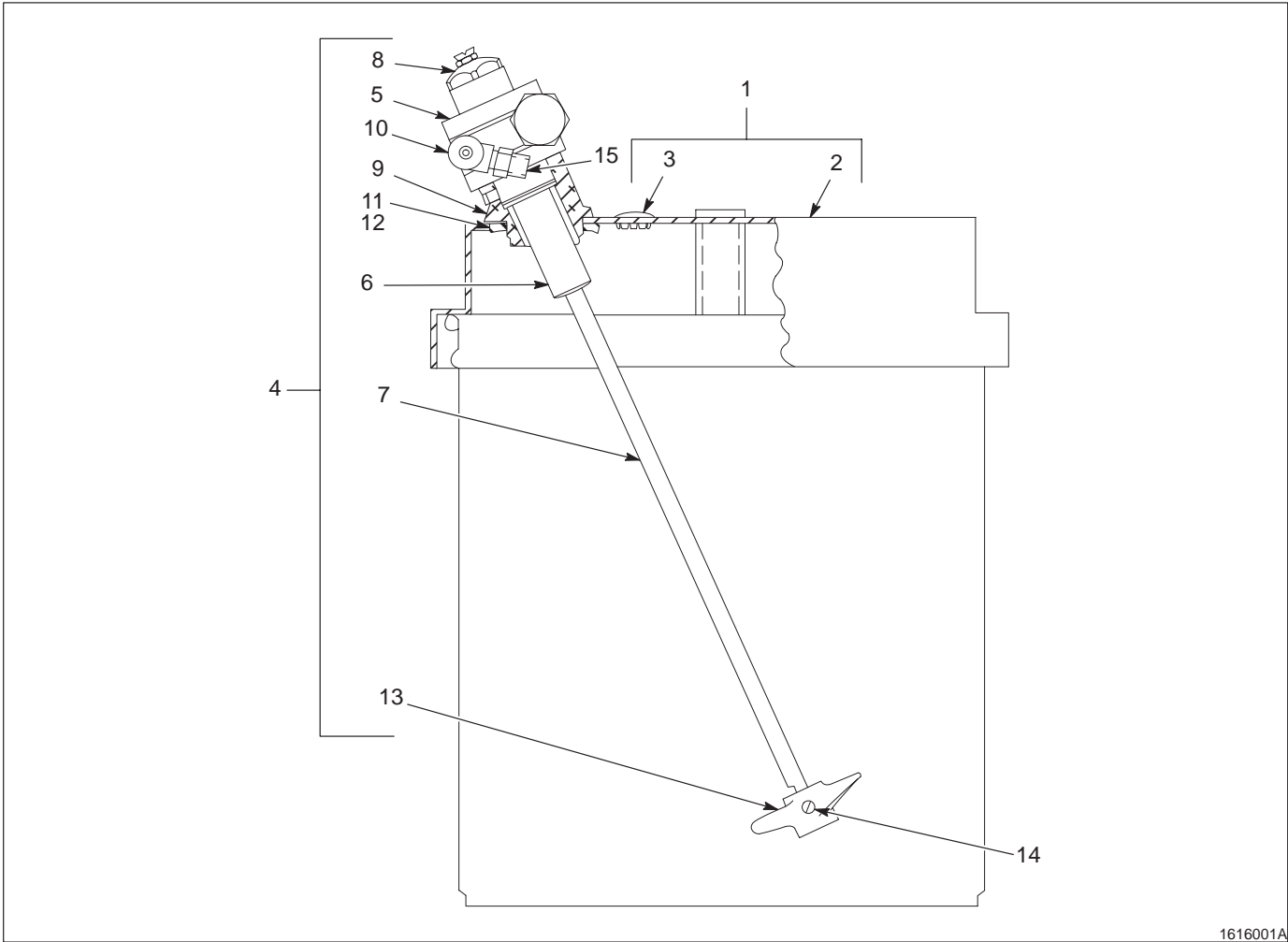
Fig. 1 5-gallon bucket agitator with cover
